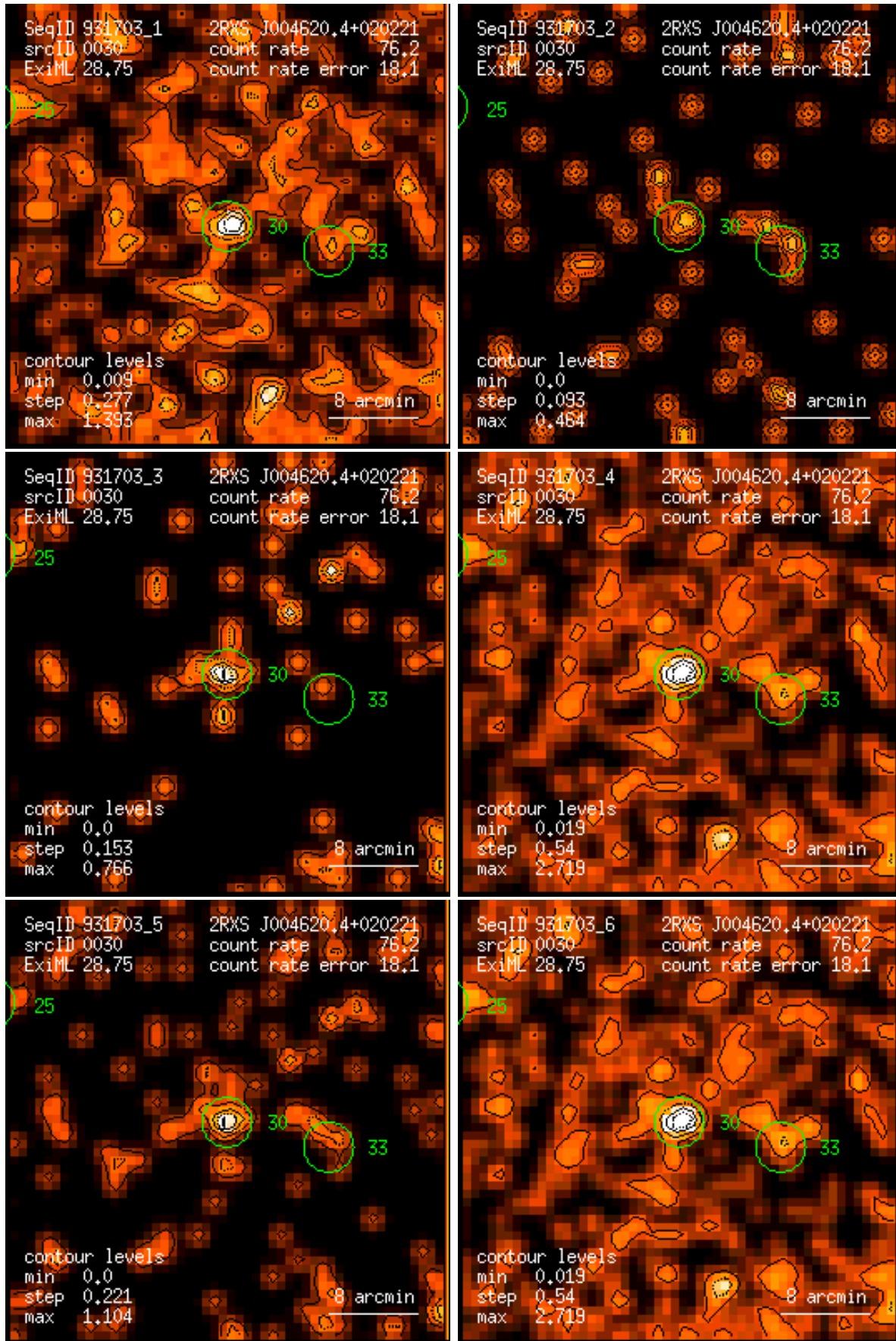
Figure 30: RASS 931703: detection 0030: band rate images, Gaussian filter: (1) PSPC channels 11 – 41, (2) 52 – 90, (3) 91 – 201, (4) 11 – 235, (5) 52 – 201, (6) 11 – 201. Broad band rates in counts/ks. Band rate contour levels in counts/ks/arcmin 2 .
