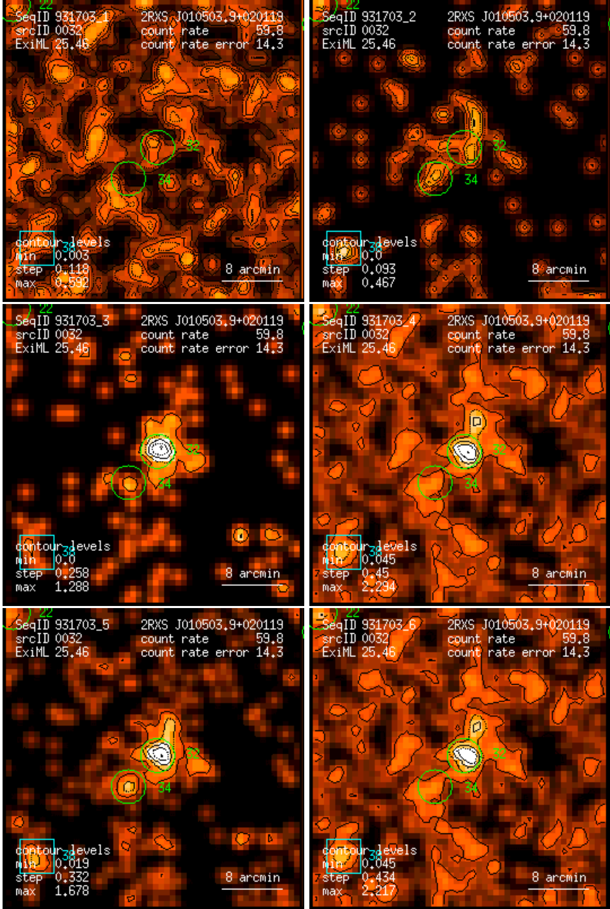
Figure 32: RASS 931703: detection 0032: band rate images, Gaussian filter: (1) PSPC channels 11 – 41, (2) 52 – 90, (3) 91 – 201, (4) 11 – 235, (5) 52 – 201, (6) 11 – 201. Broad band rates in counts/ks. Band rate contour levels in counts/ks/arcmin 2 .
