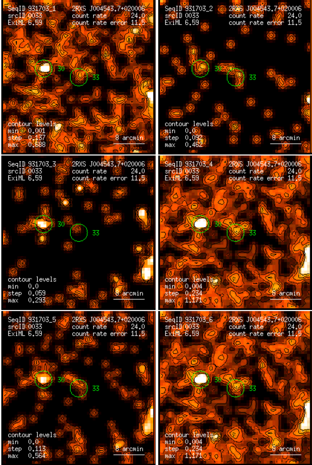
Figure 33: RASS 931703: detection 0033: band rate images, Gaussian filter: (1) PSPC channels 11 – 41, (2) 52 – 90, (3) 91 – 201, (4) 11 – 235, (5) 52 – 201, (6) 11 – 201. Broad band rates in counts/ks. Band rate contour levels in counts/ks/arcmin 2 .
