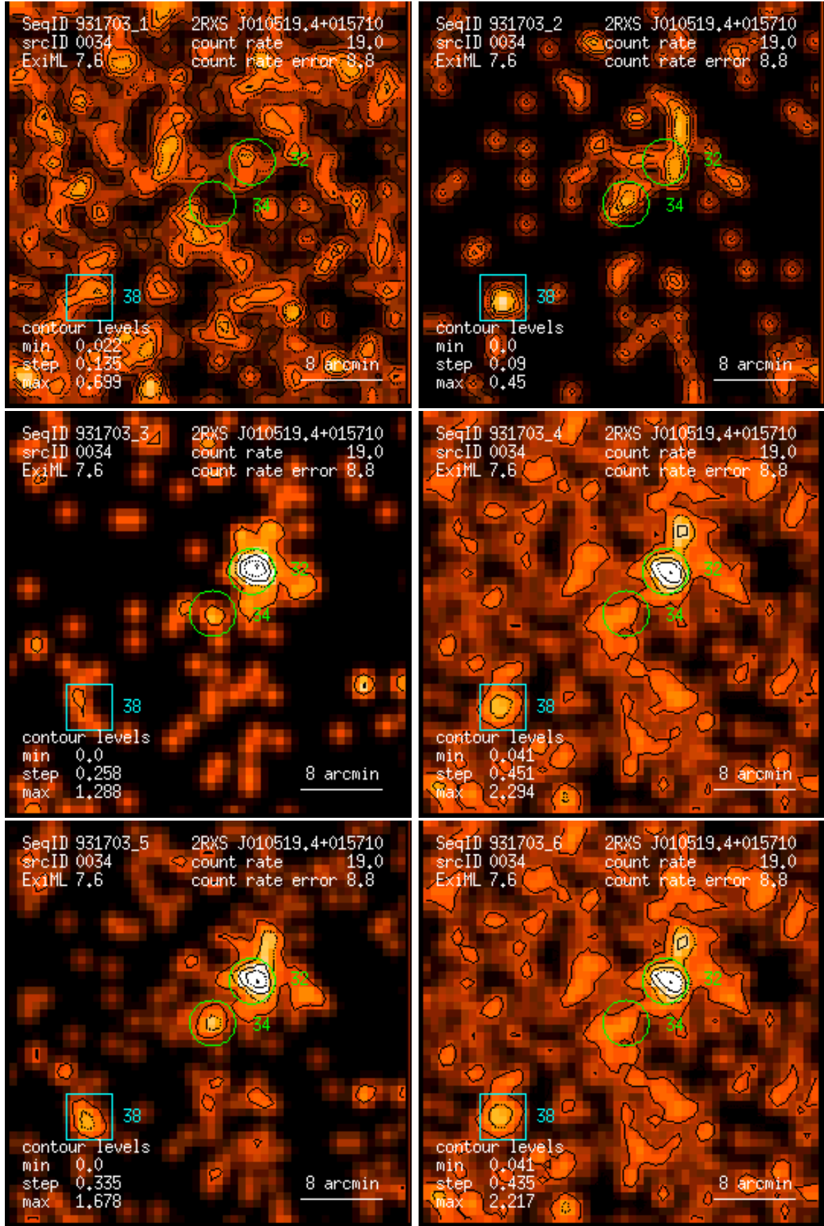
Figure 34: RASS 931703: detection 0034: band rate images, Gaussian filter: (1) PSPC channels 11 – 41, (2) 52 – 90, (3) 91 – 201, (4) 11 – 235, (5) 52 – 201, (6) 11 – 201. Broad band rates in counts/ks. Band rate contour levels in counts/ks/arcmin 2 .
