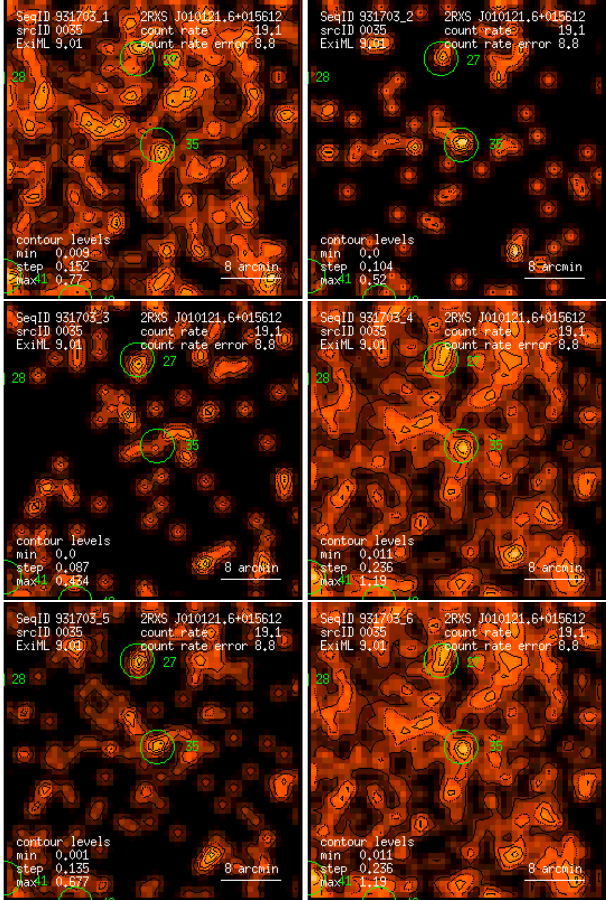
Figure 35: RASS 931703: detection 0035: band rate images, Gaussian filter: (1) PSPC channels 11 – 41, (2) 52 – 90, (3) 91 – 201, (4) 11 – 235, (5) 52 – 201, (6) 11 – 201. Broad band rates in counts/ks. Band rate contour levels in counts/ks/arcmin 2 .
