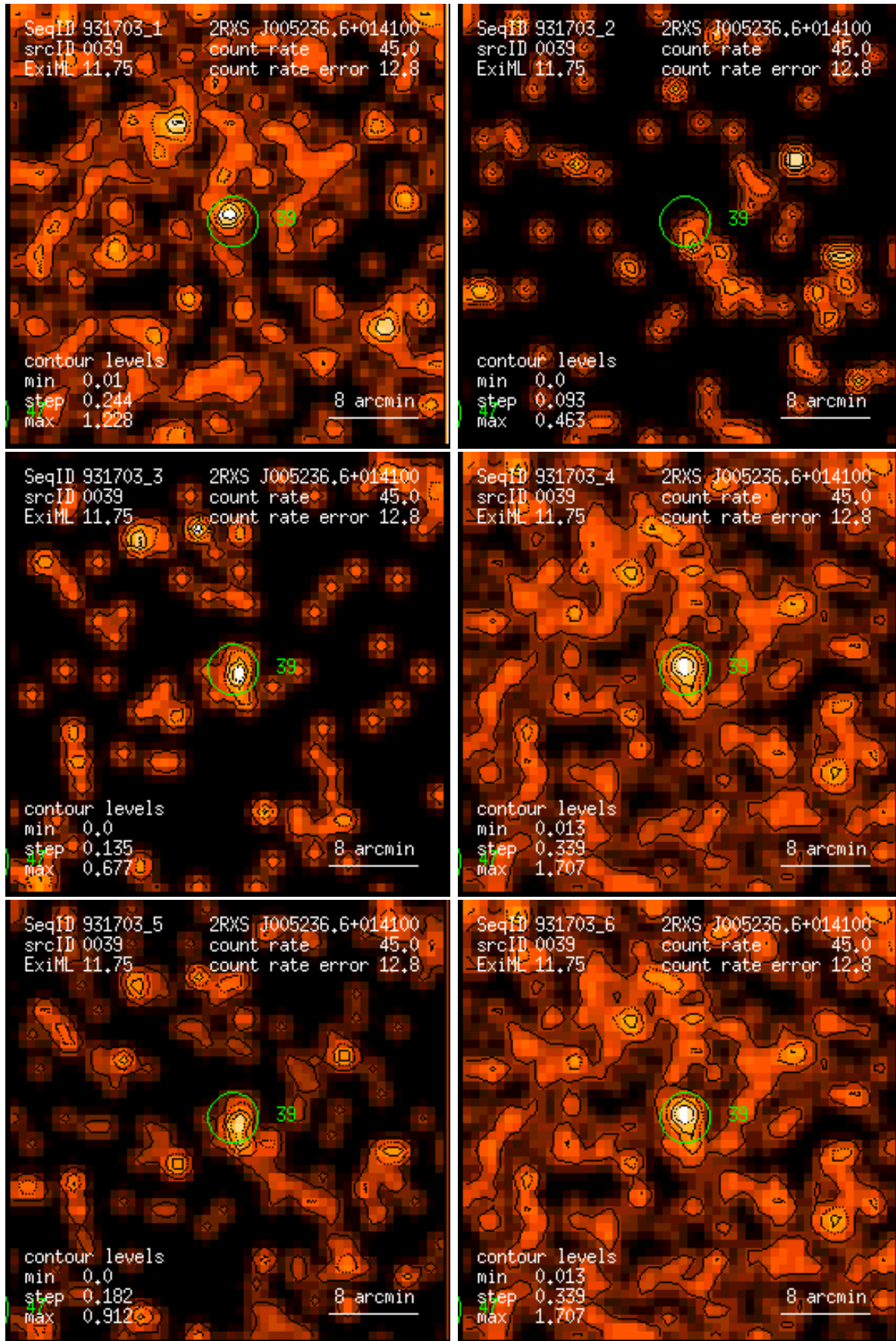
Figure 39: RASS 931703: detection 0039: band rate images, Gaussian filter: (1) PSPC channels 11 – 41, (2) 52 – 90, (3) 91 – 201, (4) 11 – 235, (5) 52 – 201, (6) 11 – 201. Broad band rates in counts/ks. Band rate contour levels in counts/ks/arcmin 2 .
