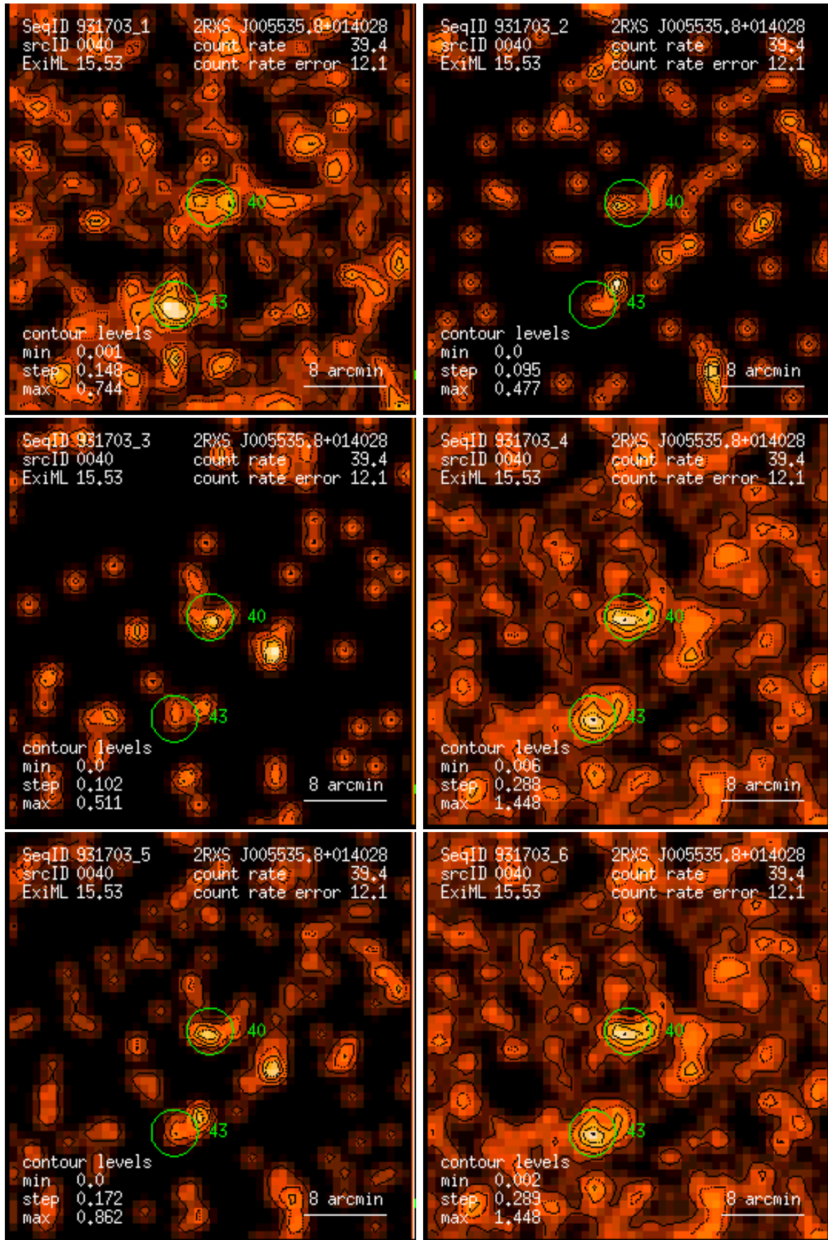
Figure 40: RASS 931703: detection 0040: band rate images, Gaussian filter: (1) PSPC channels 11 – 41, (2) 52 – 90, (3) 91 – 201, (4) 11 – 235, (5) 52 – 201, (6) 11 – 201. Broad band rates in counts/ks. Band rate contour levels in counts/ks/arcmin 2 .
