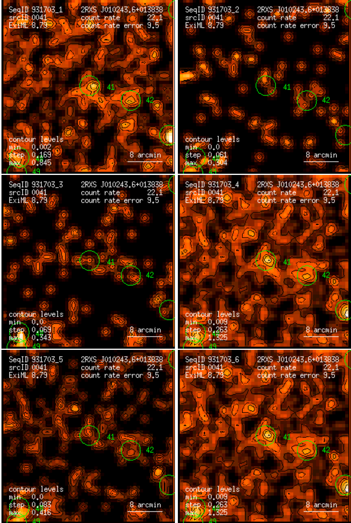
Figure 41: RASS 931703: detection 0041: band rate images, Gaussian filter: (1) PSPC channels 11 – 41, (2) 52 – 90, (3) 91 – 201, (4) 11 – 235, (5) 52 – 201, (6) 11 – 201. Broad band rates in counts/ks. Band rate contour levels in counts/ks/arcmin 2 .
