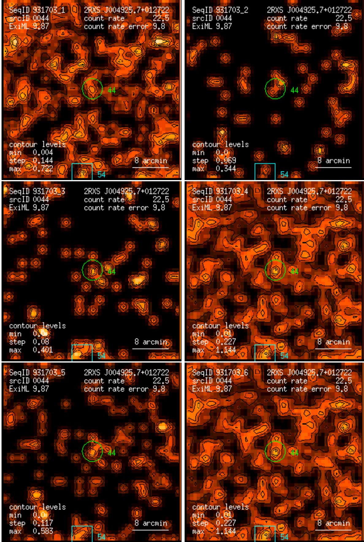
Figure 44: RASS 931703: detection 0044: band rate images, Gaussian filter: (1) PSPC channels 11 – 41, (2) 52 – 90, (3) 91 – 201, (4) 11 – 235, (5) 52 – 201, (6) 11 – 201. Broad band rates in counts/ks. Band rate contour levels in counts/ks/arcmin 2 .
