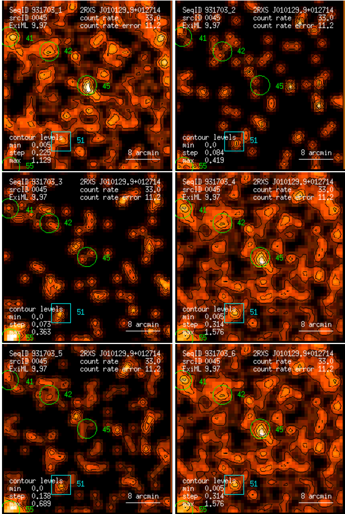
Figure 45: RASS 931703: detection 0045: band rate images, Gaussian filter: (1) PSPC channels 11 – 41, (2) 52 – 90, (3) 91 – 201, (4) 11 – 235, (5) 52 – 201, (6) 11 – 201. Broad band rates in counts/ks. Band rate contour levels in counts/ks/arcmin 2 .
