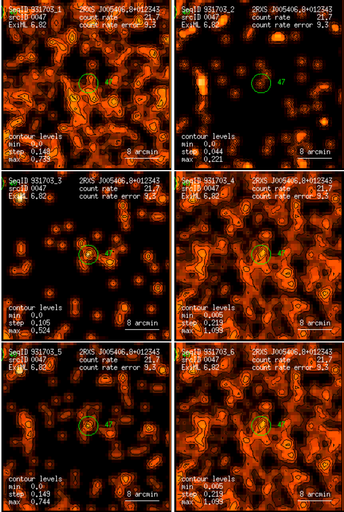
Figure 47: RASS 931703: detection 0047: band rate images, Gaussian filter: (1) PSPC channels 11 – 41, (2) 52 – 90, (3) 91 – 201, (4) 11 – 235, (5) 52 – 201, (6) 11 – 201. Broad band rates in counts/ks. Band rate contour levels in counts/ks/arcmin 2 .
