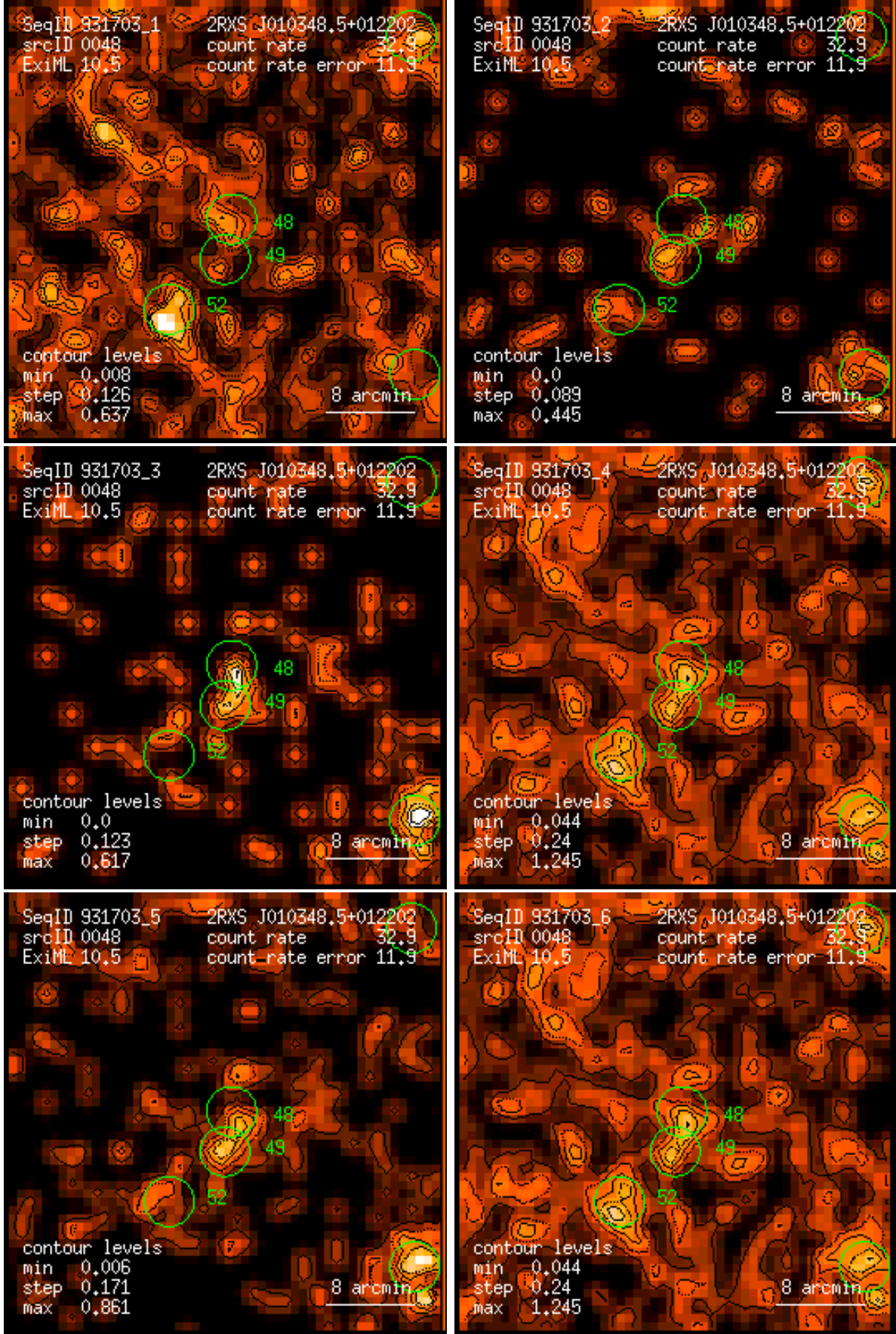
Figure 48: RASS 931703: detection 0048: band rate images, Gaussian filter: (1) PSPC channels 11 – 41, (2) 52 – 90, (3) 91 – 201, (4) 11 – 235, (5) 52 – 201, (6) 11 – 201. Broad band rates in counts/ks. Band rate contour levels in counts/ks/arcmin 2 .
