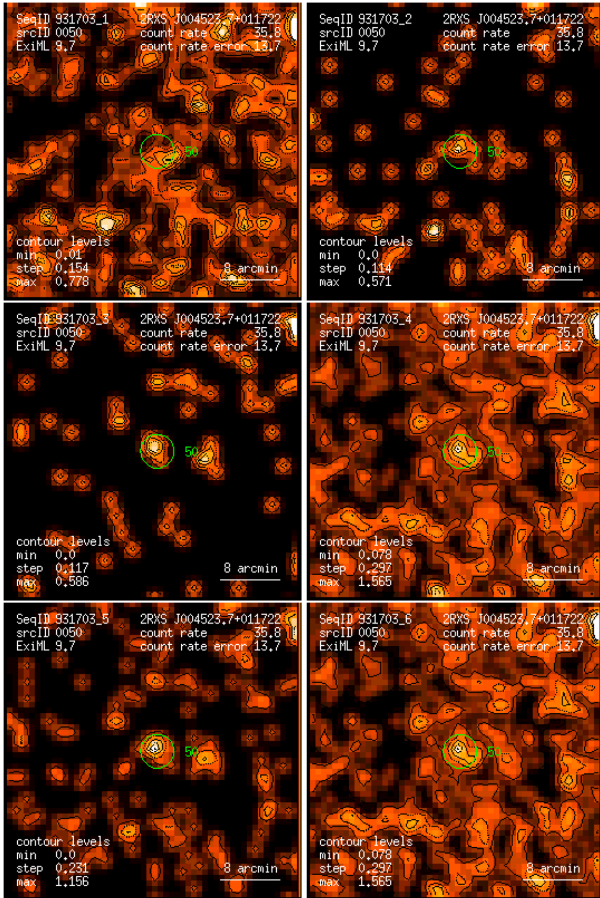
Figure 50: RASS 931703: detection 0050: band rate images, Gaussian filter: (1) PSPC channels 11 – 41, (2) 52 – 90, (3) 91 – 201, (4) 11 – 235, (5) 52 – 201, (6) 11 – 201. Broad band rates in counts/ks. Band rate contour levels in counts/ks/arcmin 2 .
