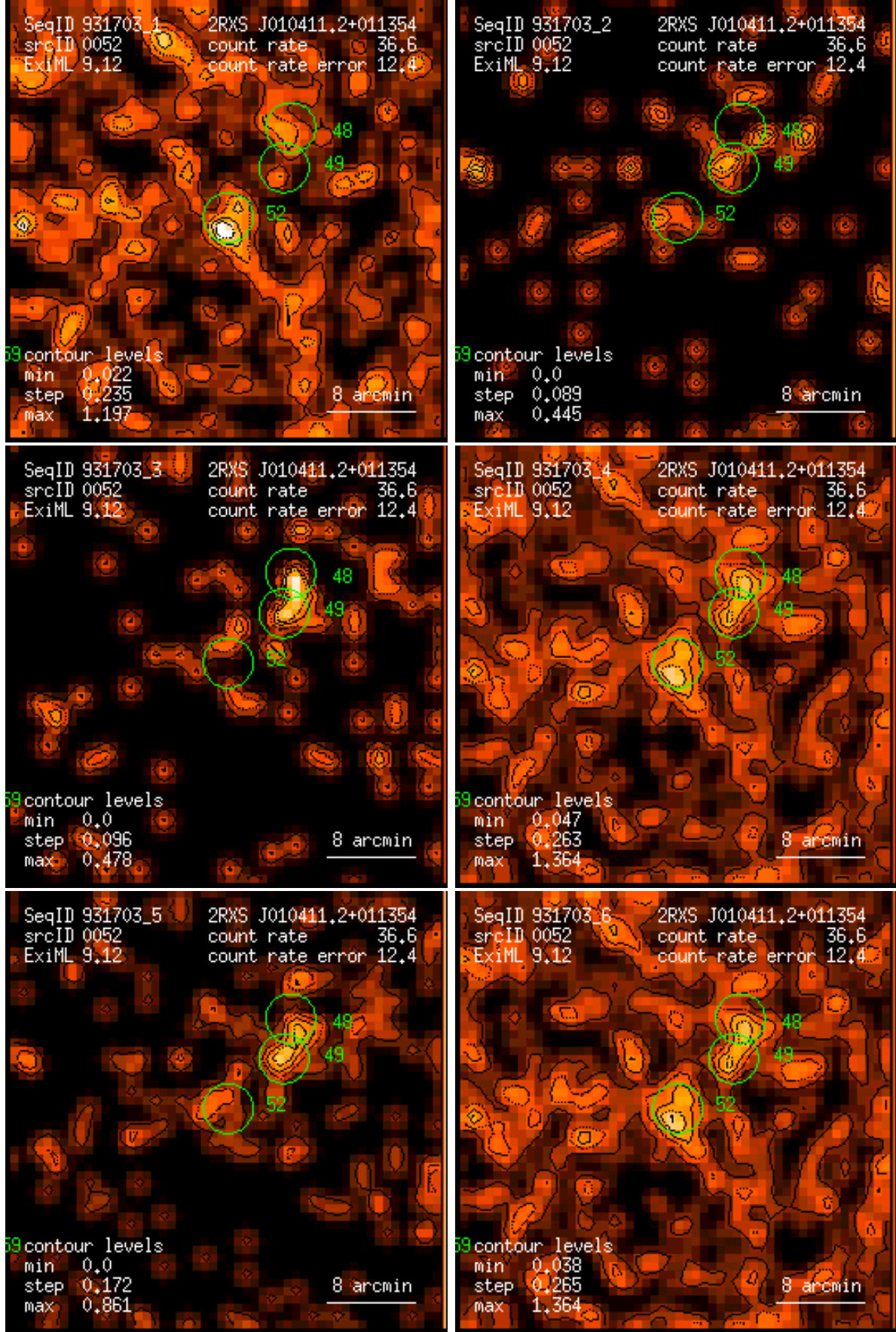
Figure 52: RASS 931703: detection 0052: band rate images, Gaussian filter: (1) PSPC channels 11 – 41, (2) 52 – 90, (3) 91 – 201, (4) 11 – 235, (5) 52 – 201, (6) 11 – 201. Broad band rates in counts/ks. Band rate contour levels in counts/ks/arcmin 2 .
