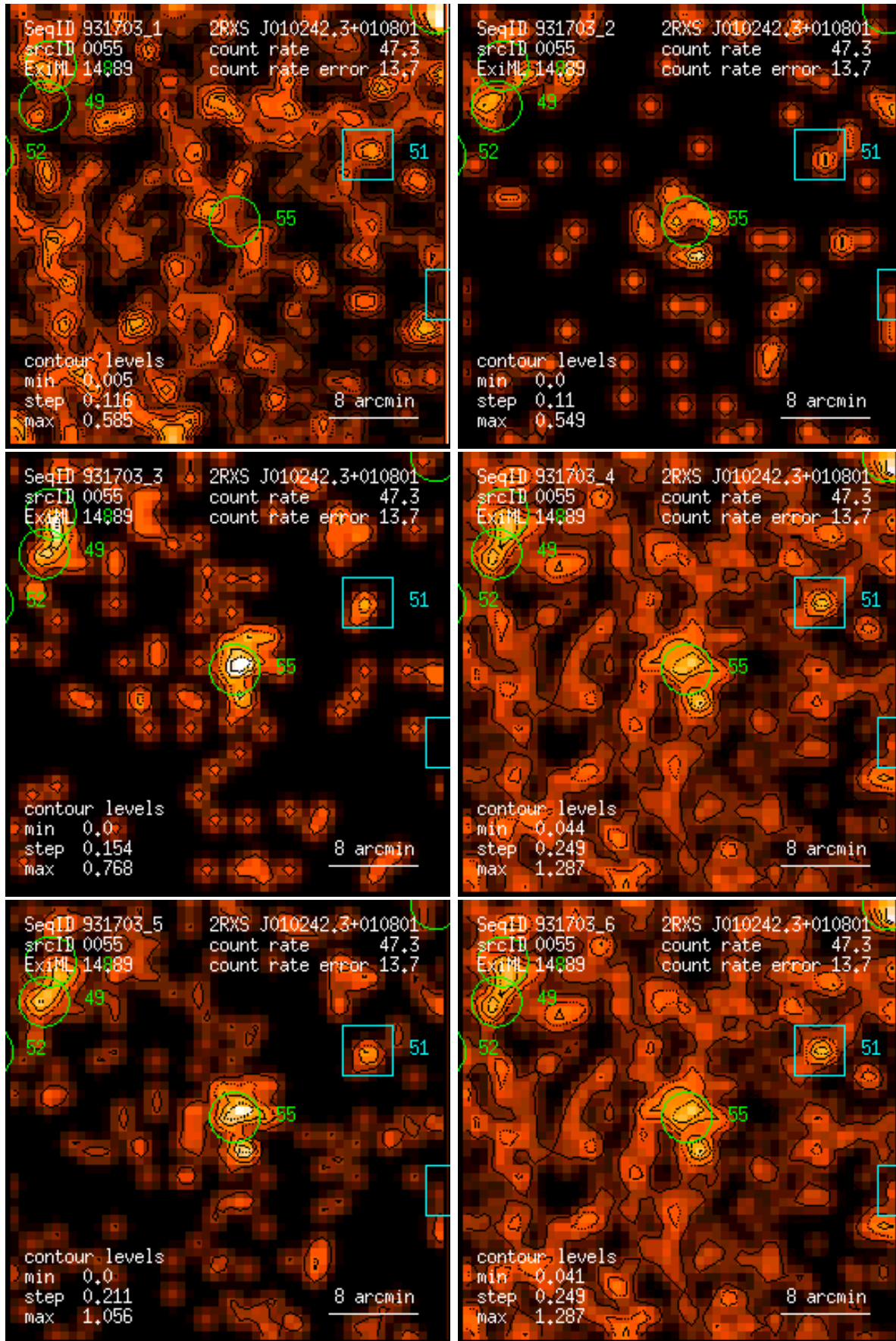
Figure 55: RASS 931703: detection 0055: band rate images, Gaussian filter: (1) PSPC channels 11 – 41, (2) 52 – 90, (3) 91 – 201, (4) 11 – 235, (5) 52 – 201, (6) 11 – 201. Broad band rates in counts/ks. Band rate contour levels in counts/ks/arcmin 2 .
