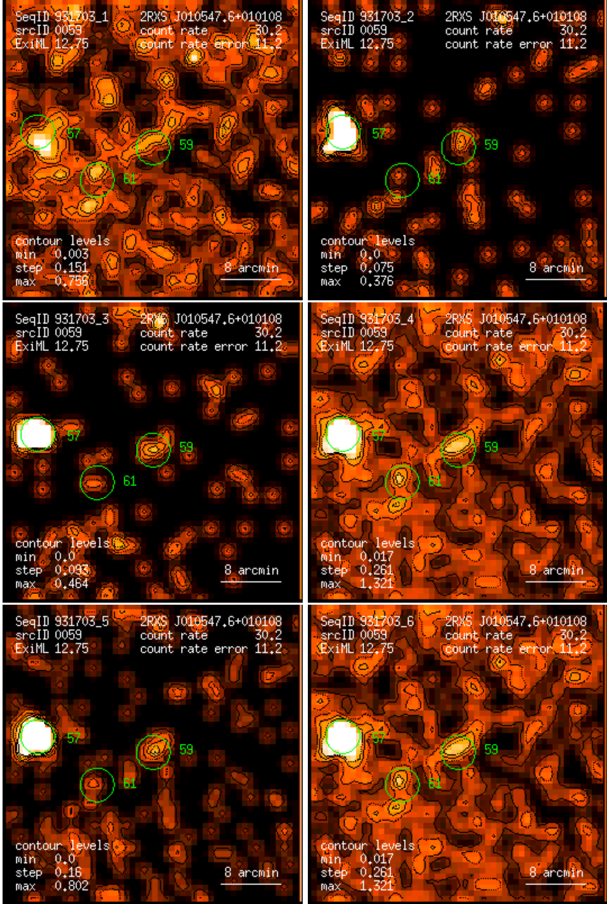
Figure 59: RASS 931703: detection 0059: band rate images, Gaussian filter: (1) PSPC channels 11 – 41, (2) 52 – 90, (3) 91 – 201, (4) 11 – 235, (5) 52 – 201, (6) 11 – 201. Broad band rates in counts/ks. Band rate contour levels in counts/ks/arcmin 2 .
