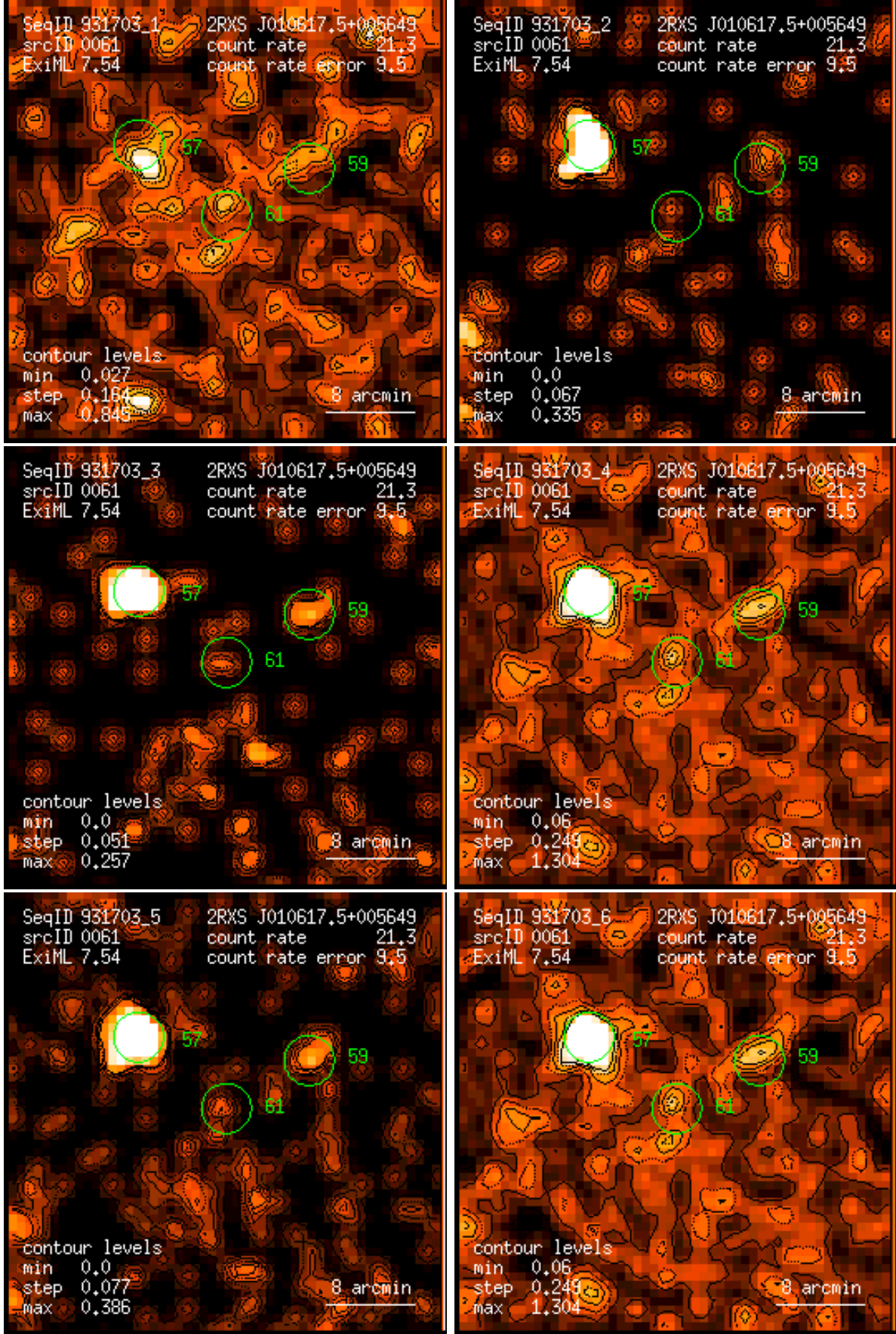
Figure 61: RASS 931703: detection 0061: band rate images, Gaussian filter: (1) PSPP channels 11 – 41, (2) 52 – 90, (3) 91 – 201, (4) 11 – 235, (5) 52 – 201, (6) 11 – 201. Broad band rates in counts/ks. Band rate contour levels in counts/ks/arcmin 2 .
