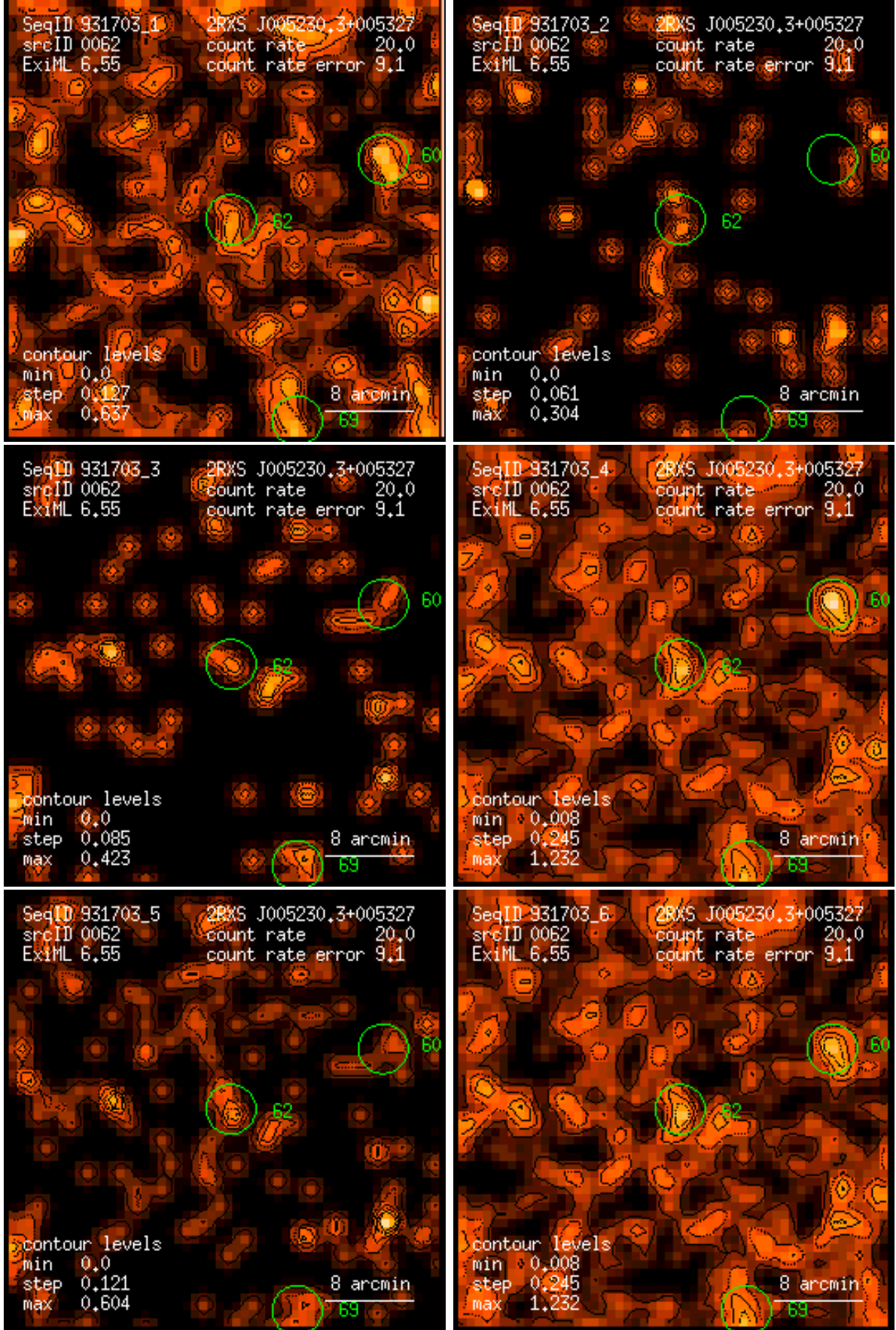
Figure 62: RASS 931703: detection 0062: band rate images, Gaussian filter: (1) PSPC channels 11 – 41, (2) 52 – 90, (3) 91 – 201, (4) 11 – 235, (5) 52 – 201, (6) 11 – 201. Broad band rates in counts/ks. Band rate contour levels in counts/ks/arcmin 2 .
