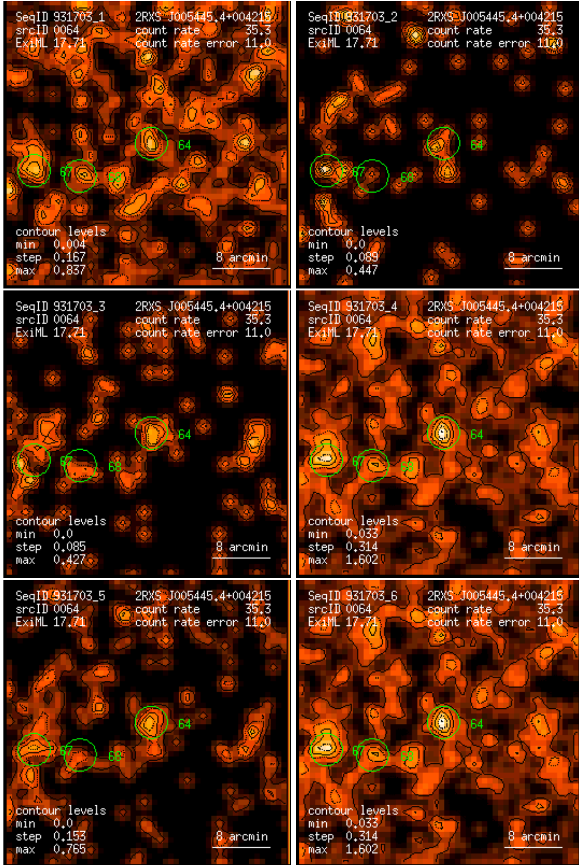
Figure 64: RASS 931703: detection 0064: band rate images, Gaussian filter: (1) PSPC channels 11 – 41, (2) 52 – 90, (3) 91 – 201, (4) 11 – 235, (5) 52 – 201, (6) 11 – 201. Broad band rates in counts/ks. Band rate contour levels in counts/ks/arcmin 2 .
