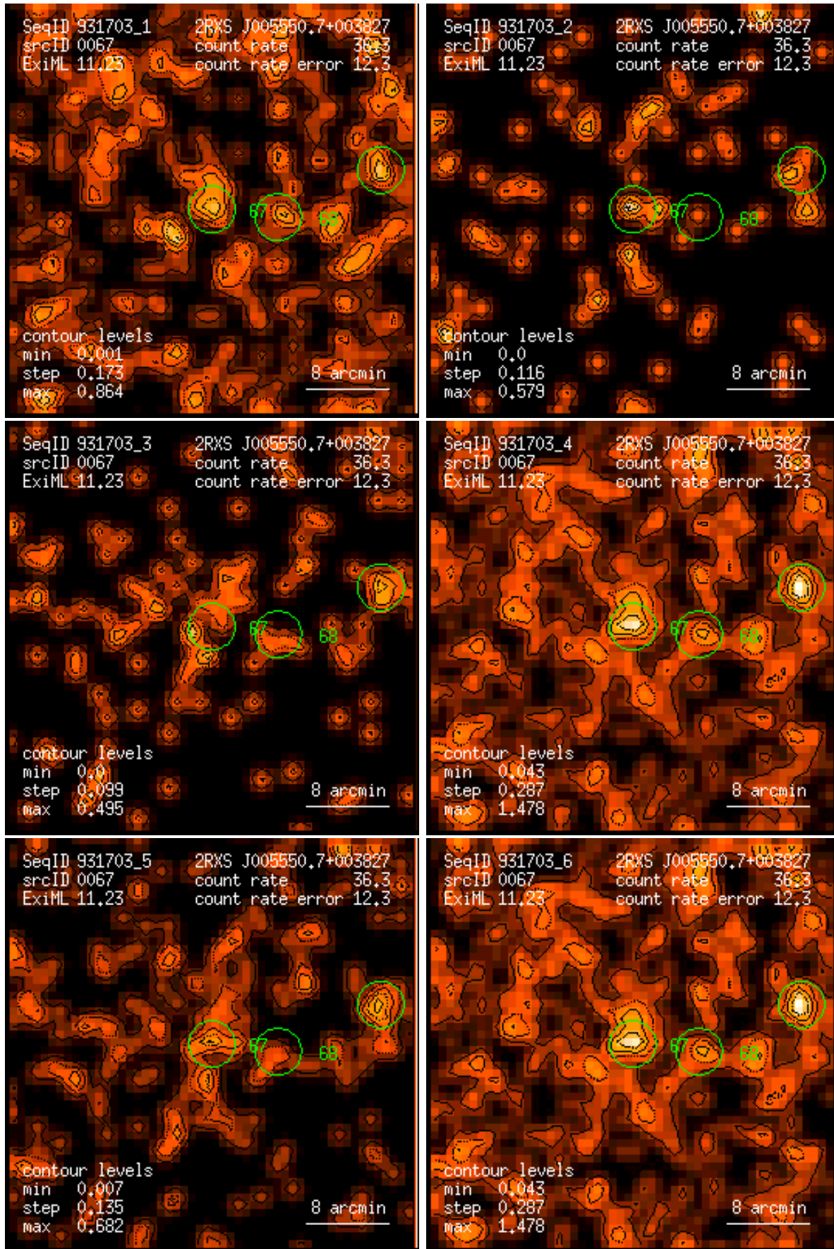
Figure 67: RASS 931703: detection 0067: band rate images, Gaussian filter: (1) PSPC channels 11 – 41, (2) 52 – 90, (3) 91 – 201, (4) 11 – 235, (5) 52 – 201, (6) 11 – 201. Broad band rates in counts/ks. Band rate contour levels in counts/ks/arcmin 2 .
