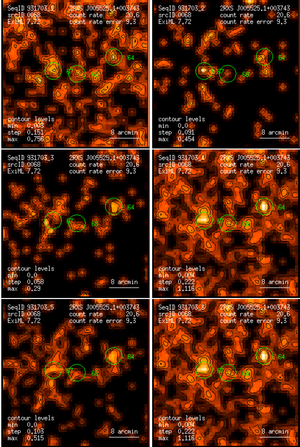
Figure 68: RASS 931703: detection 0068: band rate images, Gaussian filter: (1) PSPC channels 11 – 41, (2) 52 – 90, (3) 91 – 201, (4) 11 – 235, (5) 52 – 201, (6) 11 – 201. Broad band rates in counts/ks. Band rate contour levels in counts/ks/arcmin 2 .
