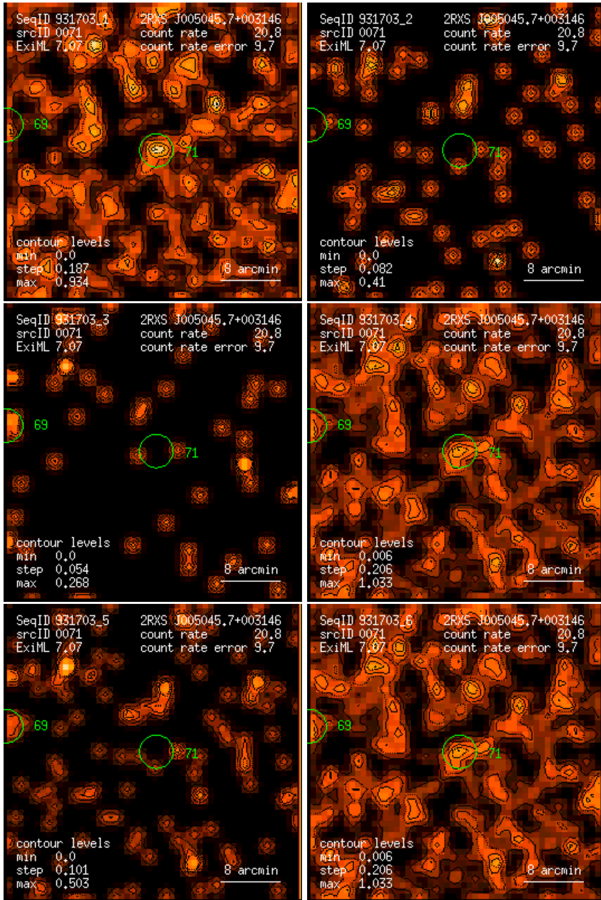
Figure 71: RASS 931703: detection 0071: band rate images, Gaussian filter: (1) PSPC channels 11 – 41, (2) 52 – 90, (3) 91 – 201, (4) 11 – 235, (5) 52 – 201, (6) 11 – 201. Broad band rates in counts/ks. Band rate contour levels in counts/ks/arcmin 2 .
