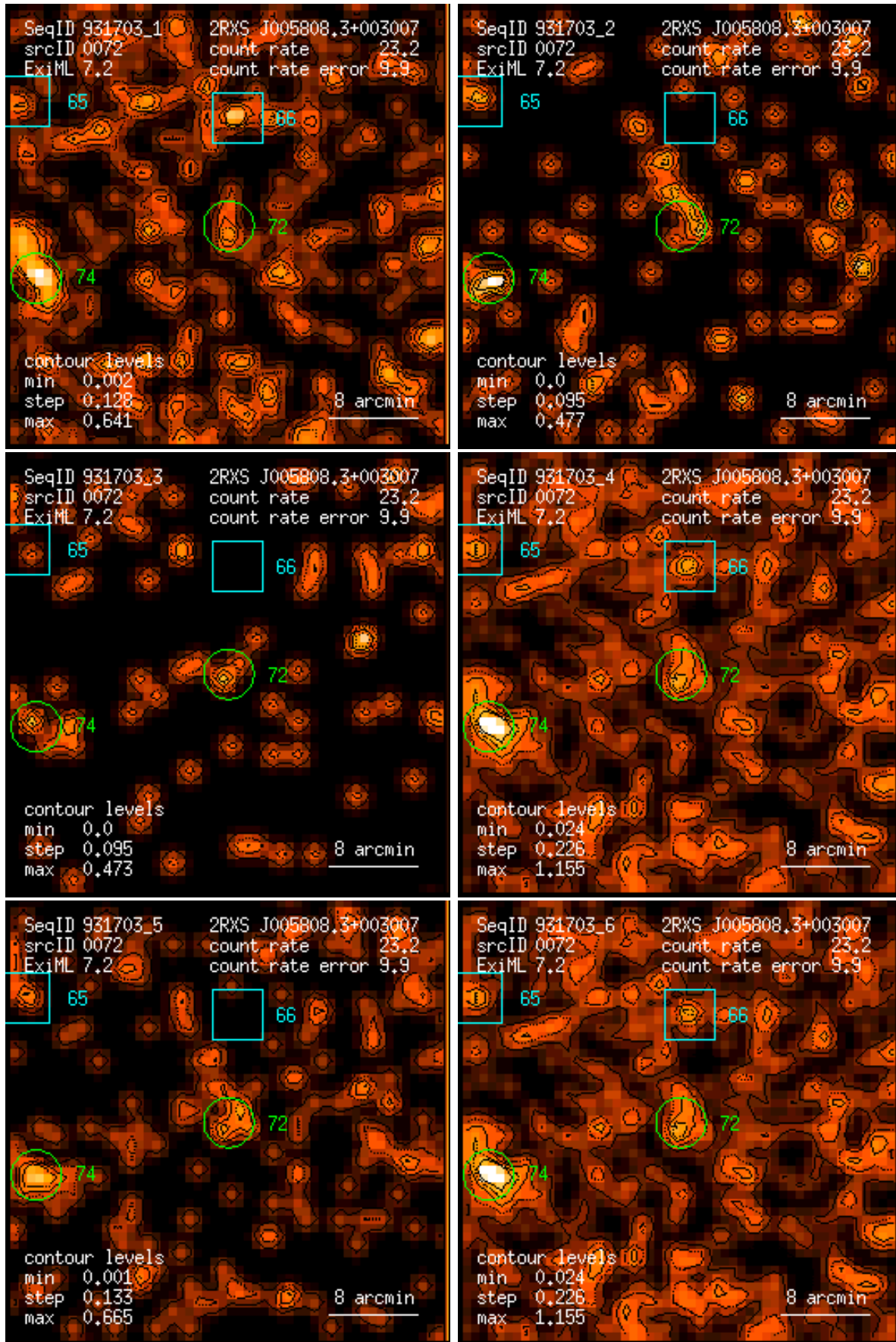
Figure 72: RASS 931703: detection 0072: band rate images, Gaussian filter: (1) PSPC channels 11 – 41, (2) 52 – 90, (3) 91 – 201, (4) 11 – 235, (5) 52 – 201, (6) 11 – 201. Broad band rates in counts/ks. Band rate contour levels in counts/ks/arcmin 2 .
