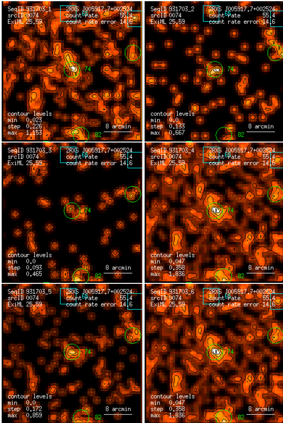
Figure 74: RASS 931703: detection 0074: band rate images, Gaussian filter: (1) PSPC channels 11 – 41, (2) 52 – 90, (3) 91 – 201, (4) 11 – 235, (5) 52 – 201, (6) 11 – 201. Broad band rates in counts/ks. Band rate contour levels in counts/ks/arcmin 2 .
