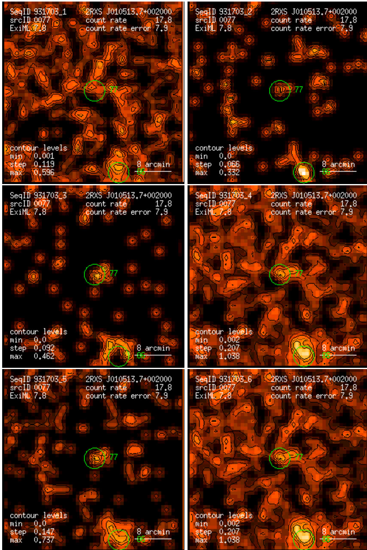
Figure 77: RASS 931703: detection 0077: band rate images, Gaussian filter: (1) PSPC channels 11 – 41, (2) 52 – 90, (3) 91 – 201, (4) 11 – 235, (5) 52 – 201, (6) 11 – 201. Broad band rates in counts/ks. Band rate contour levels in counts/ks/arcmin 2 .
