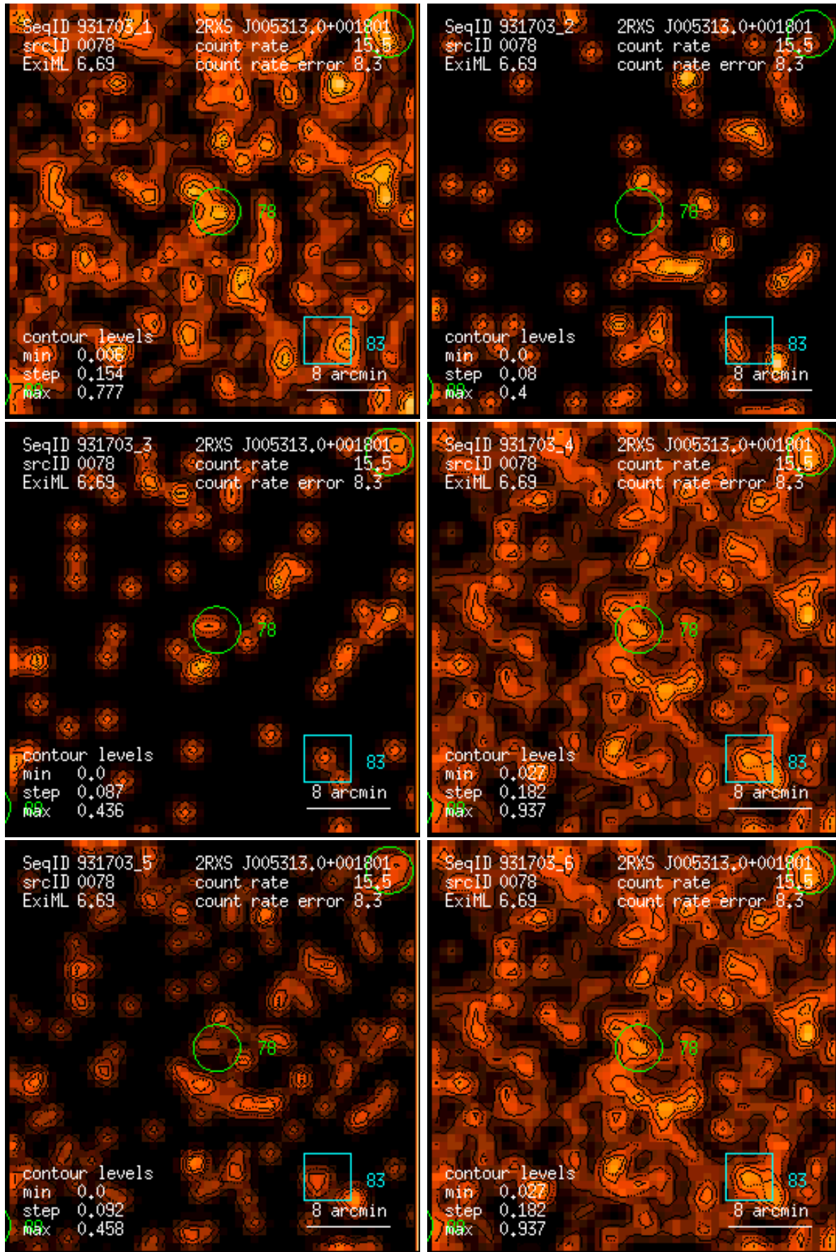
Figure 78: RASS 931703: detection 0078: band rate images, Gaussian filter: (1) PSPC channels 11 – 41, (2) 52 – 90, (3) 91 – 201, (4) 11 – 235, (5) 52 – 201, (6) 11 – 201. Broad band rates in counts/ks. Band rate contour levels in counts/ks/arcmin 2 .
