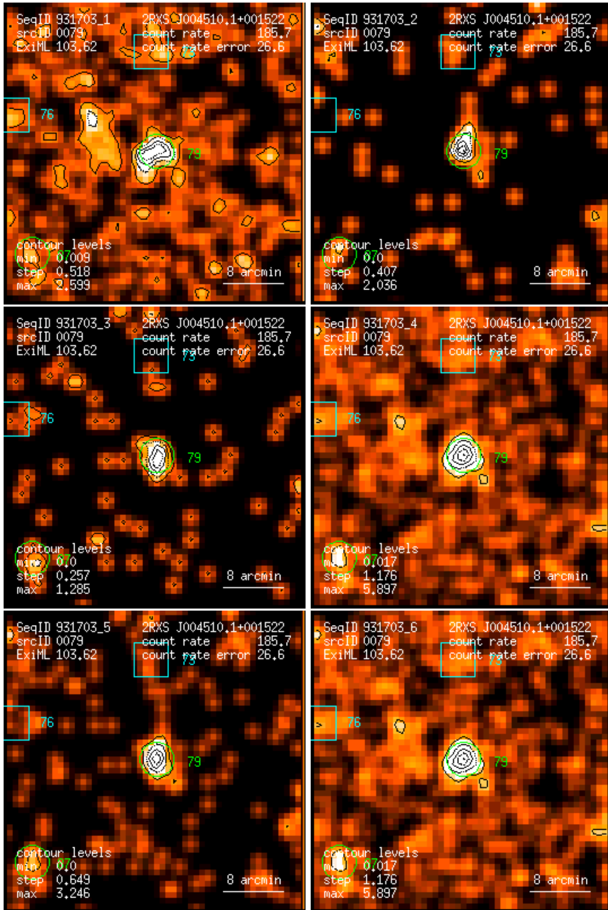
Figure 79: RASS 931703: detection 0079: band rate images, Gaussian filter: (1) PSPC channels 11 – 41, (2) 52 – 90, (3) 91 – 201, (4) 11 – 235, (5) 52 – 201, (6) 11 – 201. Broad band rates in counts/ks. Band rate contour levels in counts/ks/arcmin 2 .
