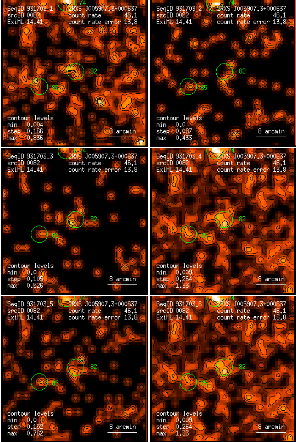
Figure 82: RASS 931703: detection 0082: band rate images, Gaussian filter: (1) PSPC channels 11 – 41, (2) 52 – 90, (3) 91 – 201, (4) 11 – 235, (5) 52 – 201, (6) 11 – 201. Broad band rates in counts/ks. Band rate contour levels in counts/ks/arcmin 2 .
