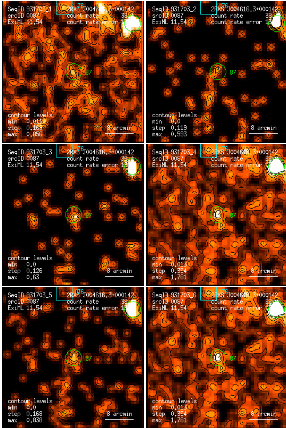
Figure 87: RASS 931703: detection 0087: band rate images, Gaussian filter: (1) PSPC channels 11 – 41, (2) 52 – 90, (3) 91 – 201, (4) 11 – 235, (5) 52 – 201, (6) 11 – 201. Broad band rates in counts/ks. Band rate contour levels in counts/ks/arcmin 2 .
