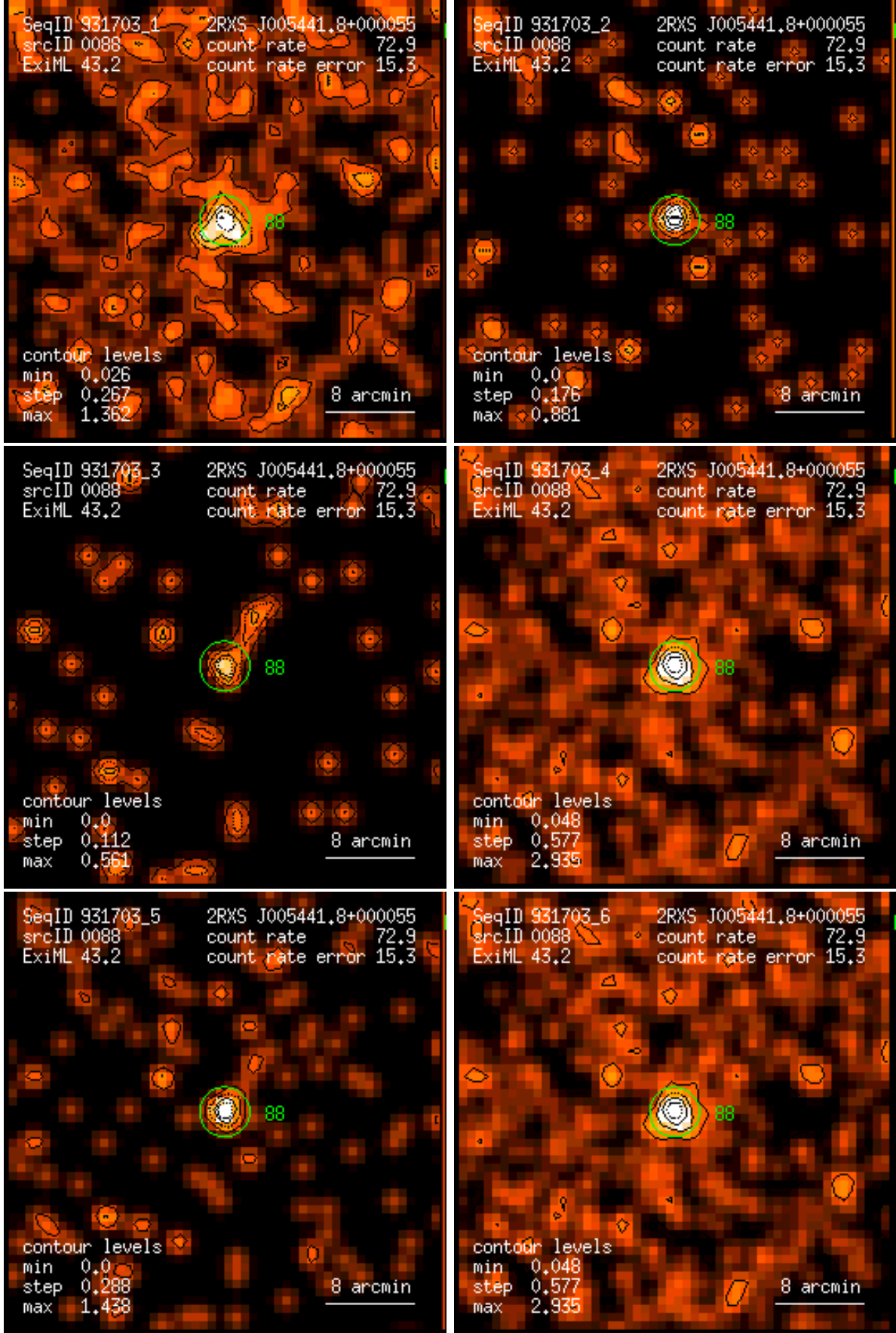
Figure 88: RASS 931703: detection 0088: band rate images, Gaussian filter: (1) PSPC channels 11 – 41, (2) 52 – 90, (3) 91 – 201, (4) 11 – 235, (5) 52 – 201, (6) 11 – 201. Broad band rates in counts/ks. Band rate contour levels in counts/ks/arcmin 2 .
