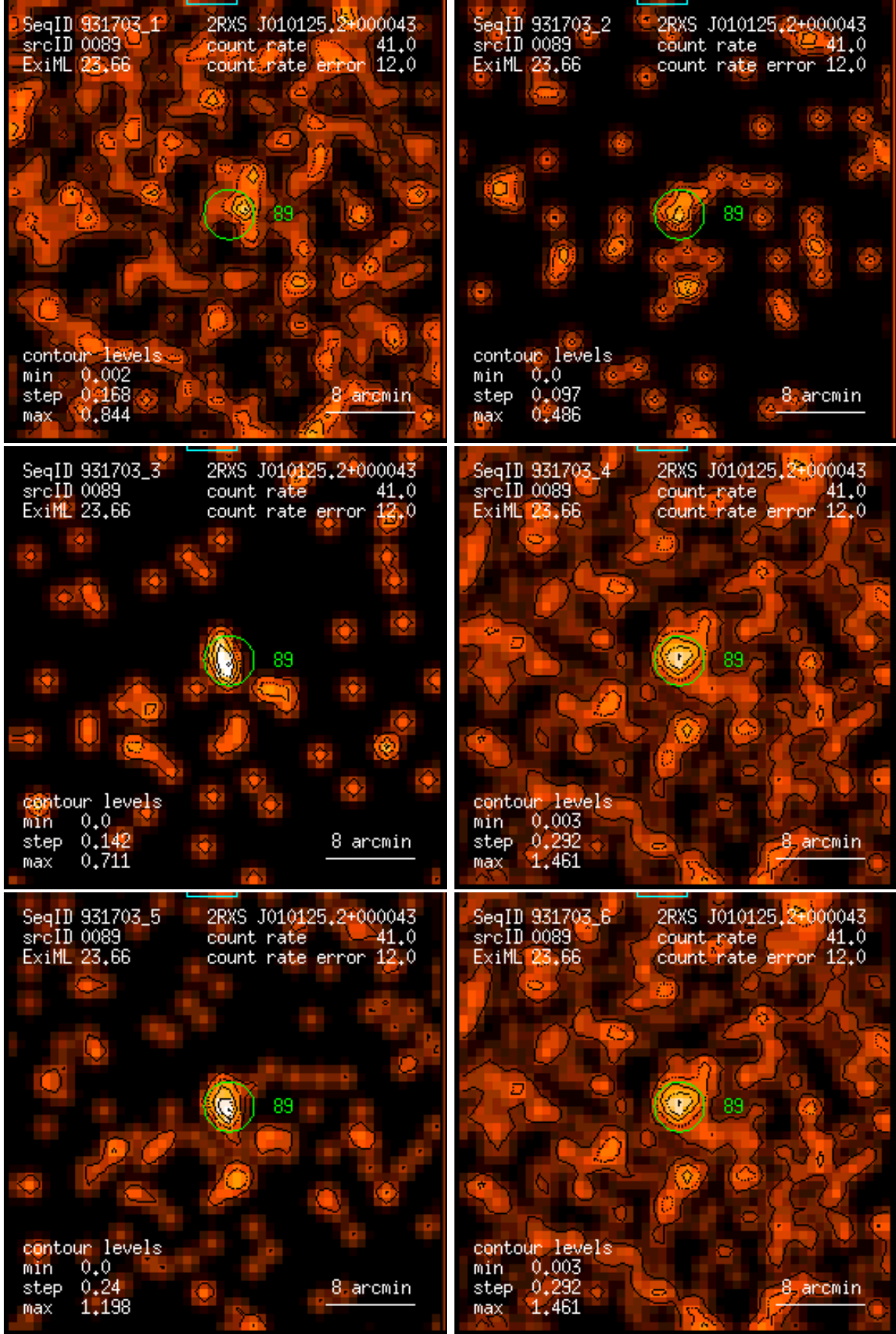
Figure 89: RASS 931703: detection 0089: band rate images, Gaussian filter: (1) PSPC channels 11 – 41, (2) 52 – 90, (3) 91 – 201, (4) 11 – 235, (5) 52 – 201, (6) 11 – 201. Broad band rates in counts/ks. Band rate contour levels in counts/ks/arcmin 2 .
