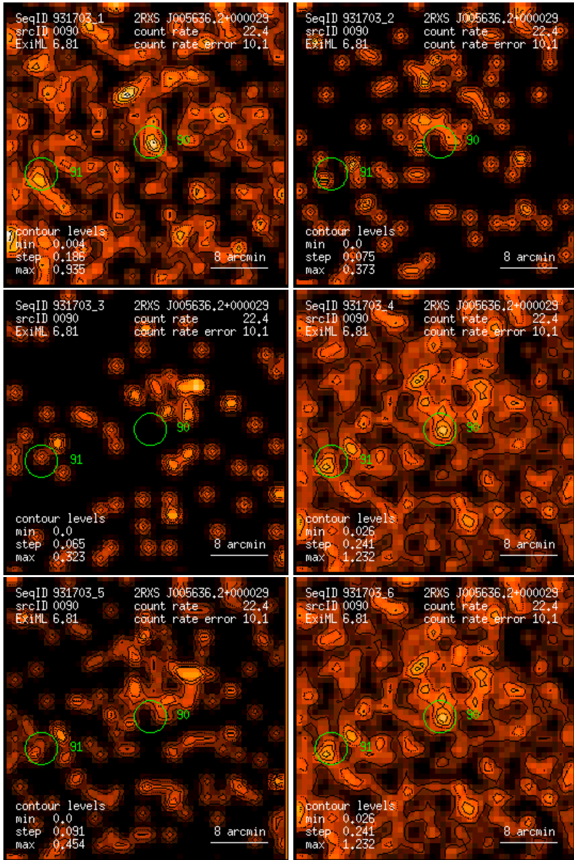
Figure 90: RASS 931703: detection 0090: band rate images, Gaussian filter: (1) PSPC channels 11 – 41, (2) 52 – 90, (3) 91 – 201, (4) 11 – 235, (5) 52 – 201, (6) 11 – 201. Broad band rates in counts/ks. Band rate contour levels in counts/ks/arcmin 2 .
