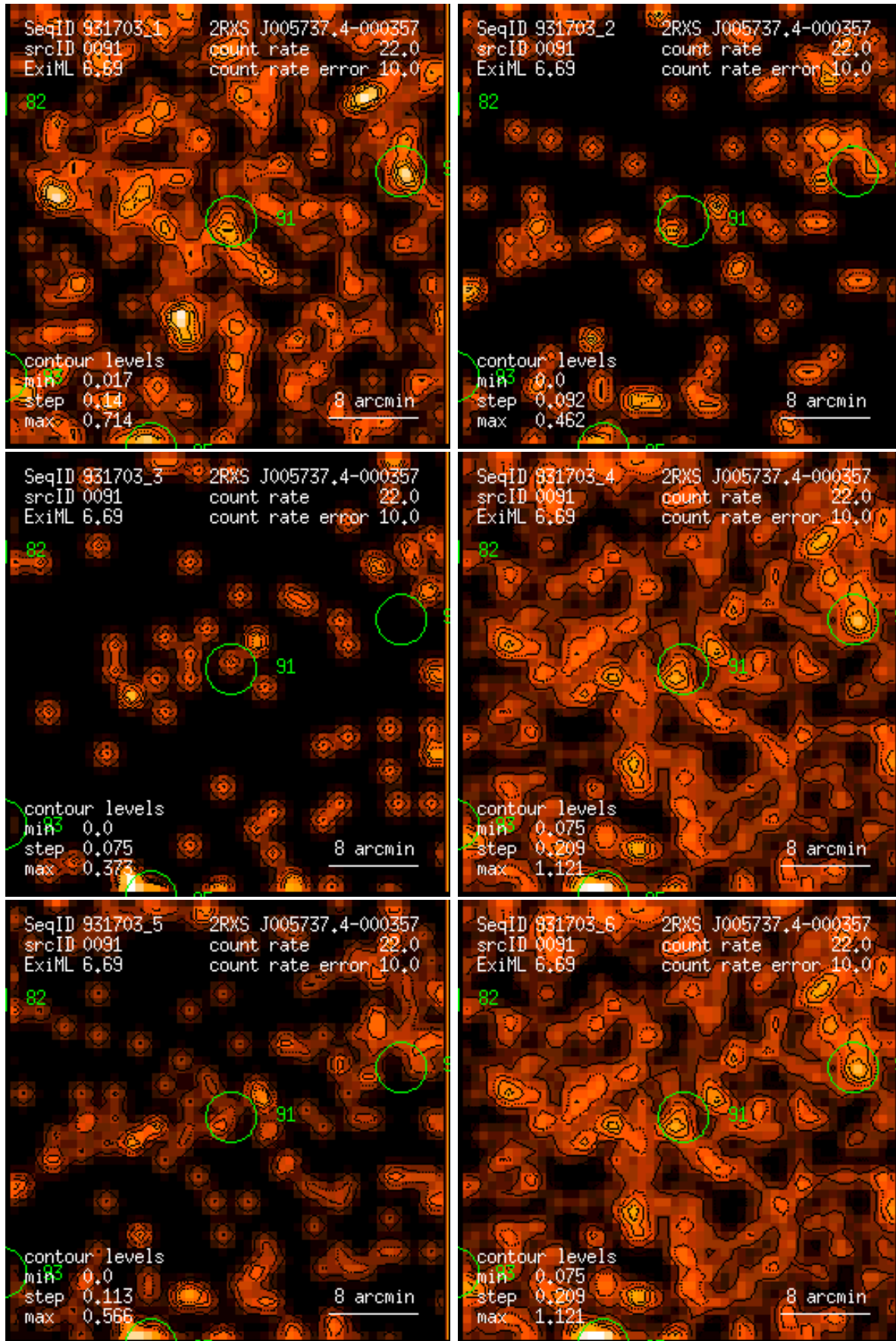
Figure 91: RASS 931703: detection 0091: band rate images, Gaussian filter: (1) PSPC channels 11 – 41, (2) 52 – 90, (3) 91 – 201, (4) 11 – 235, (5) 52 – 201, (6) 11 – 201. Broad band rates in counts/ks. Band rate contour levels in counts/ks/arcmin 2 .
