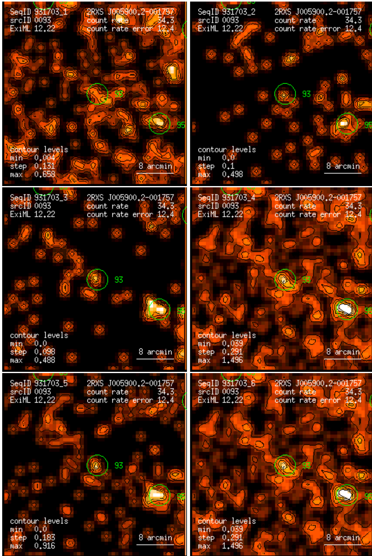
Figure 93: RASS 931703: detection 0093: band rate images, Gaussian filter: (1) PSPC channels 11 – 41, (2) 52 – 90, (3) 91 – 201, (4) 11 – 235, (5) 52 – 201, (6) 11 – 201. Broad band rates in counts/ks. Band rate contour levels in counts/ks/arcmin 2 .
