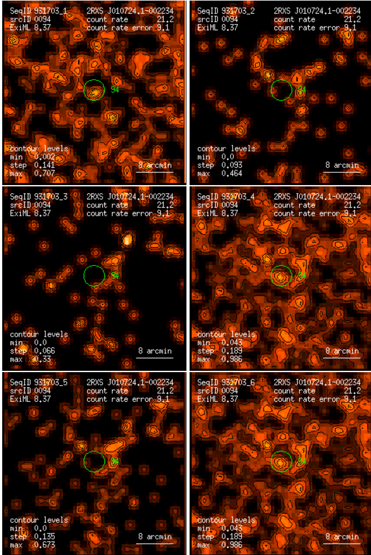
Figure 94: RASS 931703: detection 0094: band rate images, Gaussian filter: (1) PSPC channels 11 – 41, (2) 52 – 90, (3) 91 – 201, (4) 11 – 235, (5) 52 – 201, (6) 11 – 201. Broad band rates in counts/ks. Band rate contour levels in counts/ks/arcmin 2 .
