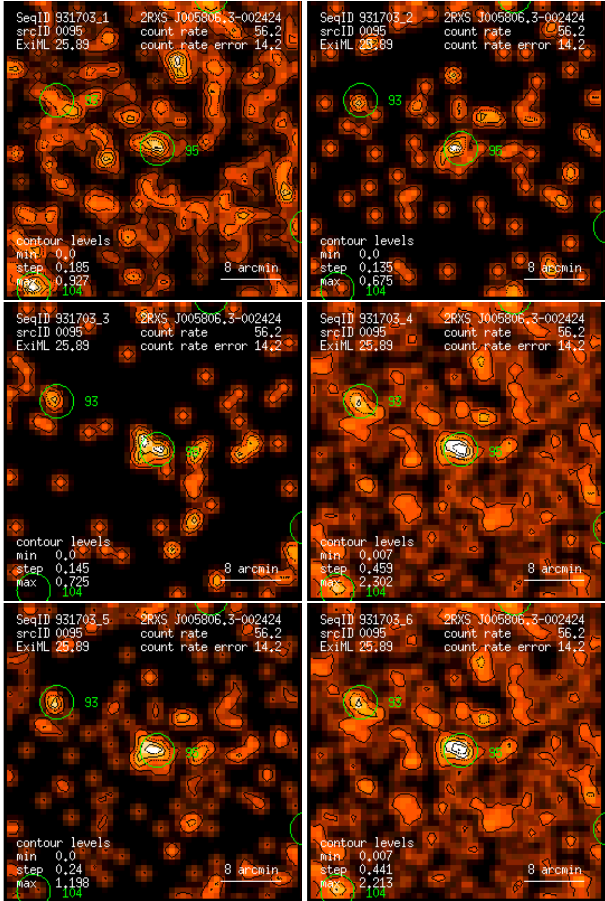
Figure 95: RASS 931703: detection 0095: band rate images, Gaussian filter: (1) PSPC channels 11 – 41, (2) 52 – 90, (3) 91 – 201, (4) 11 – 235, (5) 52 – 201, (6) 11 – 201. Broad band rates in counts/ks. Band rate contour levels in counts/ks/arcmin 2 .
