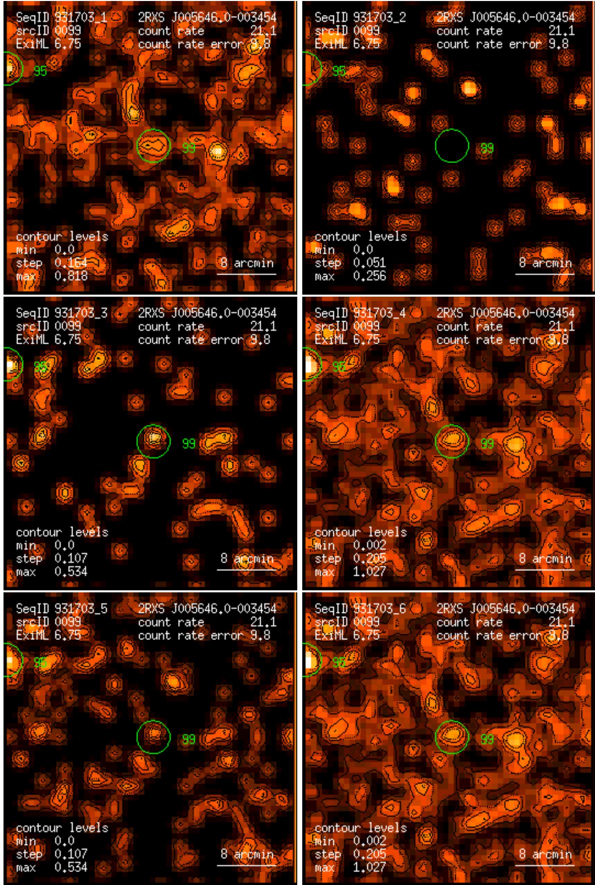
Figure 99: RASS 931703: detection 0099: band rate images, Gaussian filter: (1) PSPC channels 11 – 41, (2) 52 – 90, (3) 91 – 201, (4) 11 – 235, (5) 52 – 201, (6) 11 – 201. Broad band rates in counts/ks. Band rate contour levels in counts/ks/arcmin 2 .
