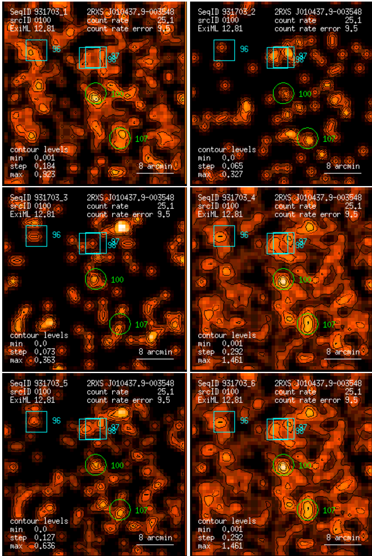
Figure 100: RASS 931703: detection 0100: band rate images, Gaussian filter: (1) PSPC channels 11 – 41, (2) 52 – 90, (3) 91 – 201, (4) 11 – 235, (5) 52 – 201, (6) 11 – 201. Broad band rates in counts/ks. Band rate contour levels in counts/ks/arcmin 2 .
