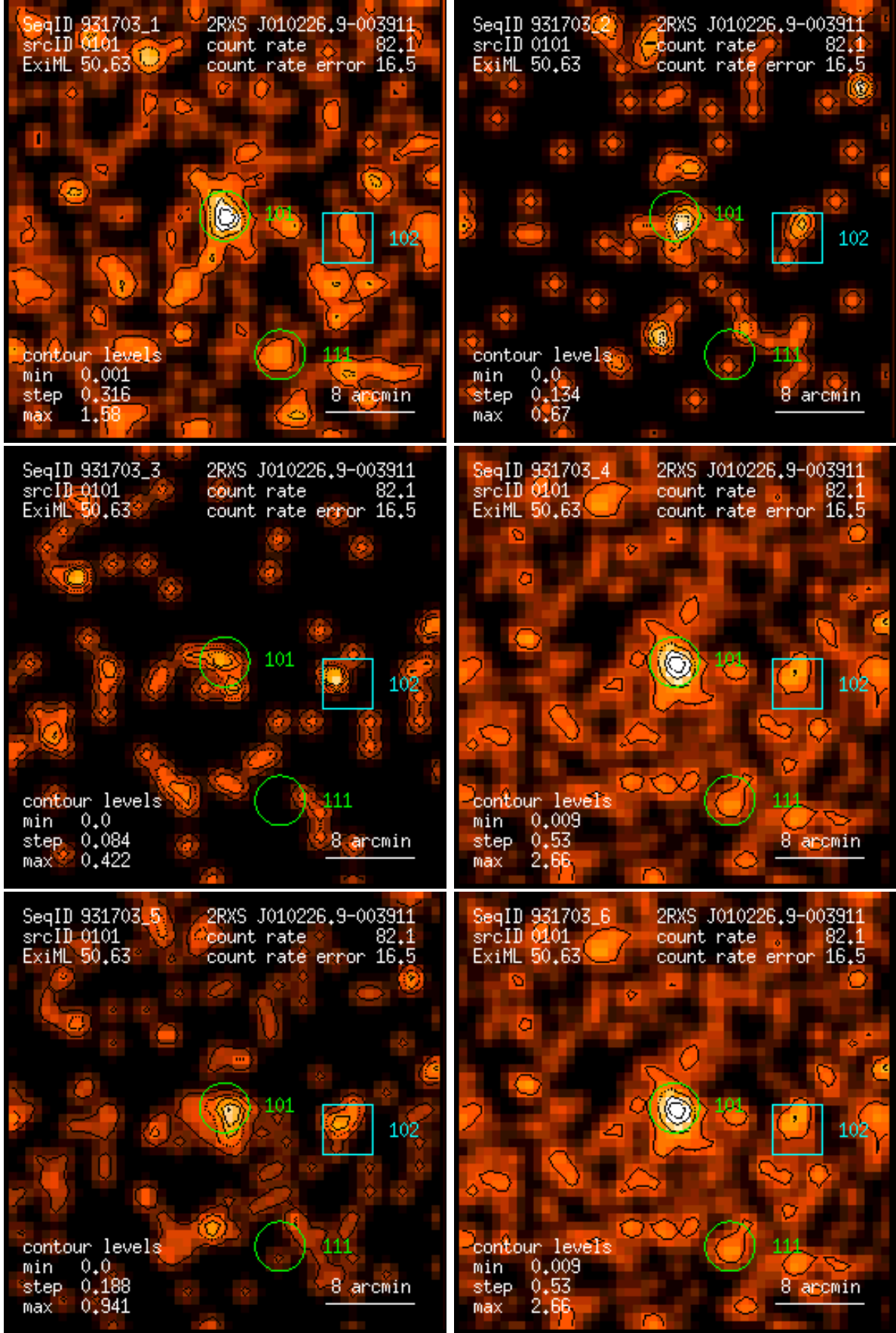
Figure 101: RASS 931703: detection 0101: band rate images, Gaussian filter: (1) PSPC channels 11 – 41, (2) 52 – 90, (3) 91 – 201, (4) 11 – 235, (5) 52 – 201, (6) 11 – 201. Broad band rates in counts/ks. Band rate contour levels in counts/ks/arcmin 2 .
