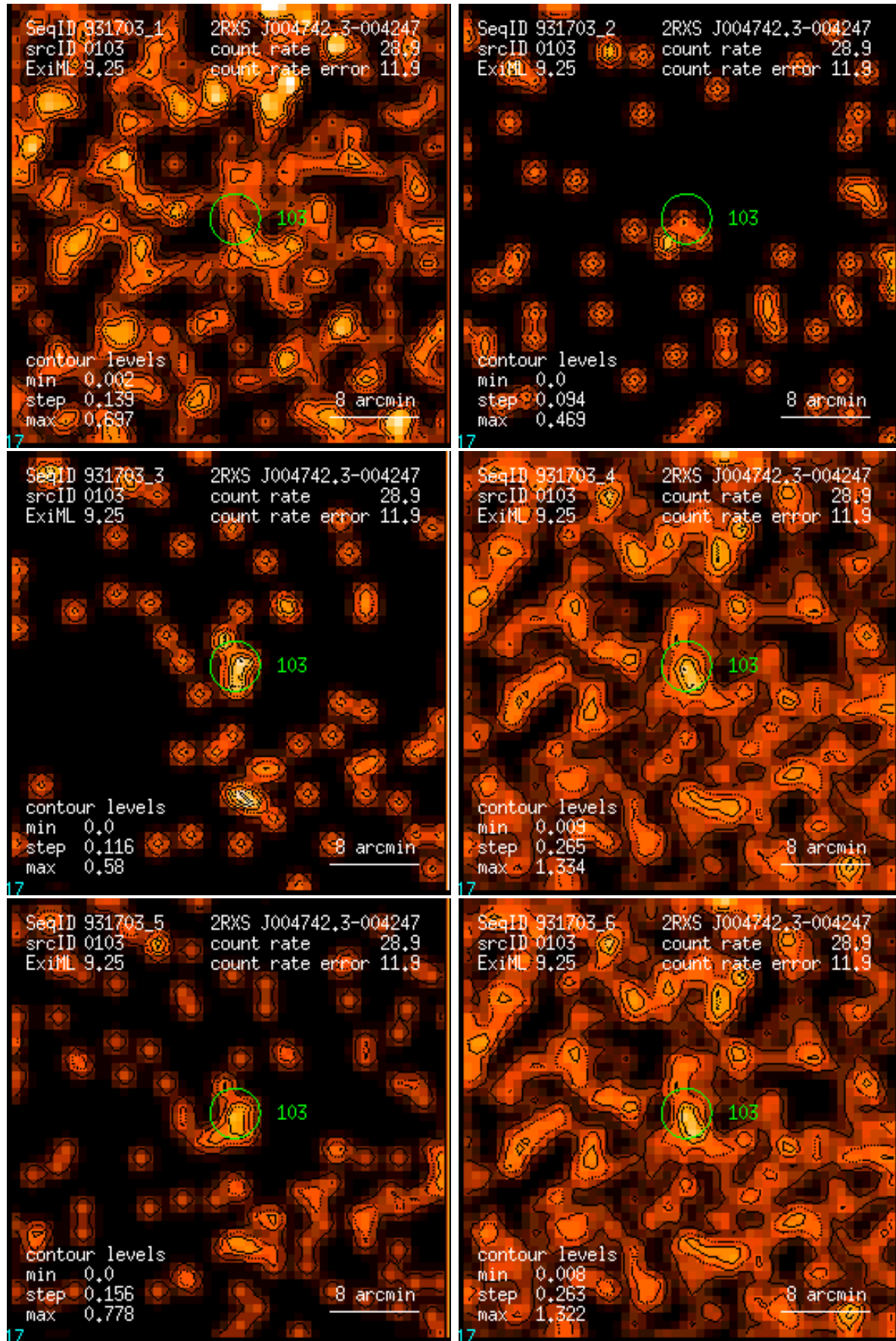
Figure 103: RASS 931703: detection 0103: band rate images, Gaussian filter: (1) PSPC channels 11 – 41, (2) 52 – 90, (3) 91 – 201, (4) 11 – 235, (5) 52 – 201, (6) 11 – 201. Broad band rates in counts/ks. Band rate contour levels in counts/ks/arcmin 2 .
