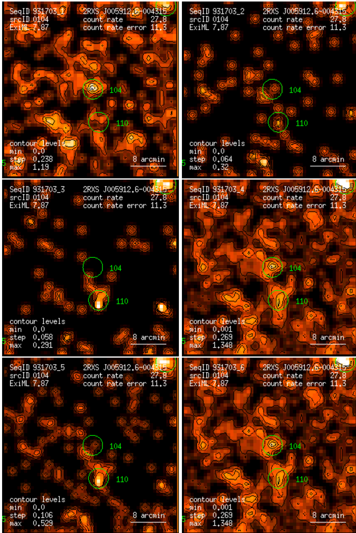
Figure 104: RASS 931703: detection 0104: band rate images, Gaussian filter: (1) PSPC channels 11 – 41, (2) 52 – 90, (3) 91 – 201, (4) 11 – 235, (5) 52 – 201, (6) 11 – 201. Broad band rates in counts/ks. Band rate contour levels in counts/ks/arcmin 2 .
