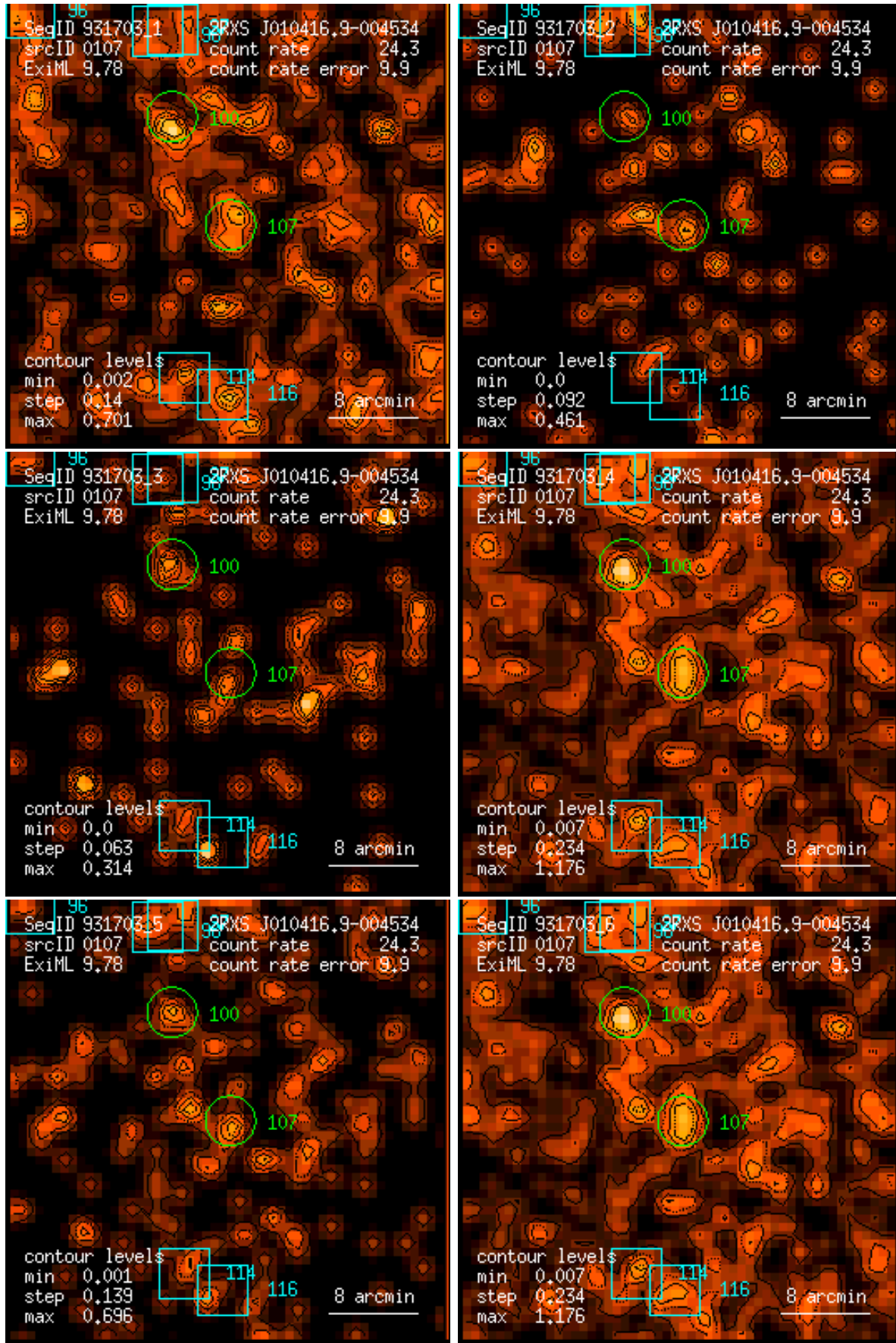
Figure 107: RASS 931703: detection 0107: band rate images, Gaussian filter: (1) PSPC channels 11 – 41, (2) 52 – 90, (3) 91 – 201, (4) 11 – 235, (5) 52 – 201, (6) 11 – 201. Broad band rates in counts/ks. Band rate contour levels in counts/ks/arcmin 2 .
