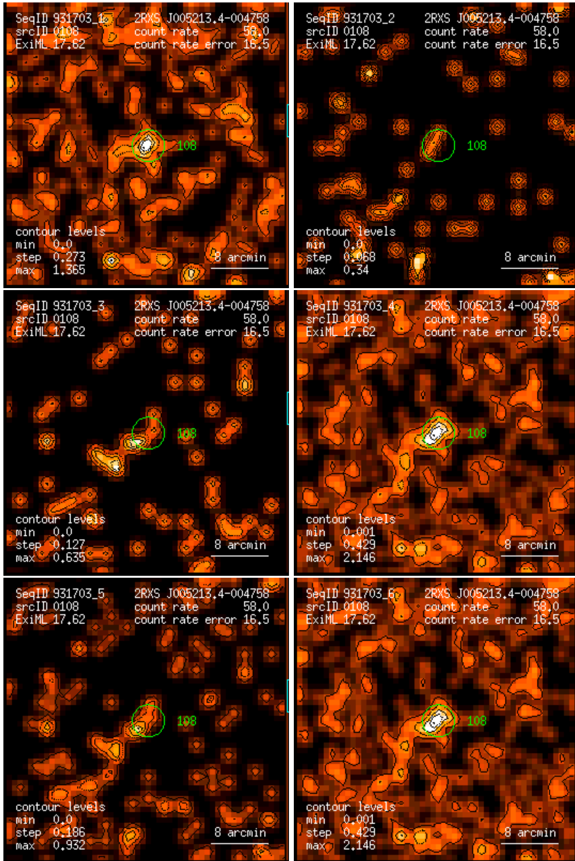
Figure 108: RASS 931703: detection 0108: band rate images, Gaussian filter: (1) PSPC channels 11 – 41, (2) 52 – 90, (3) 91 – 201, (4) 11 – 235, (5) 52 – 201, (6) 11 – 201. Broad band rates in counts/ks. Band rate contour levels in counts/ks/arcmin 2 .
