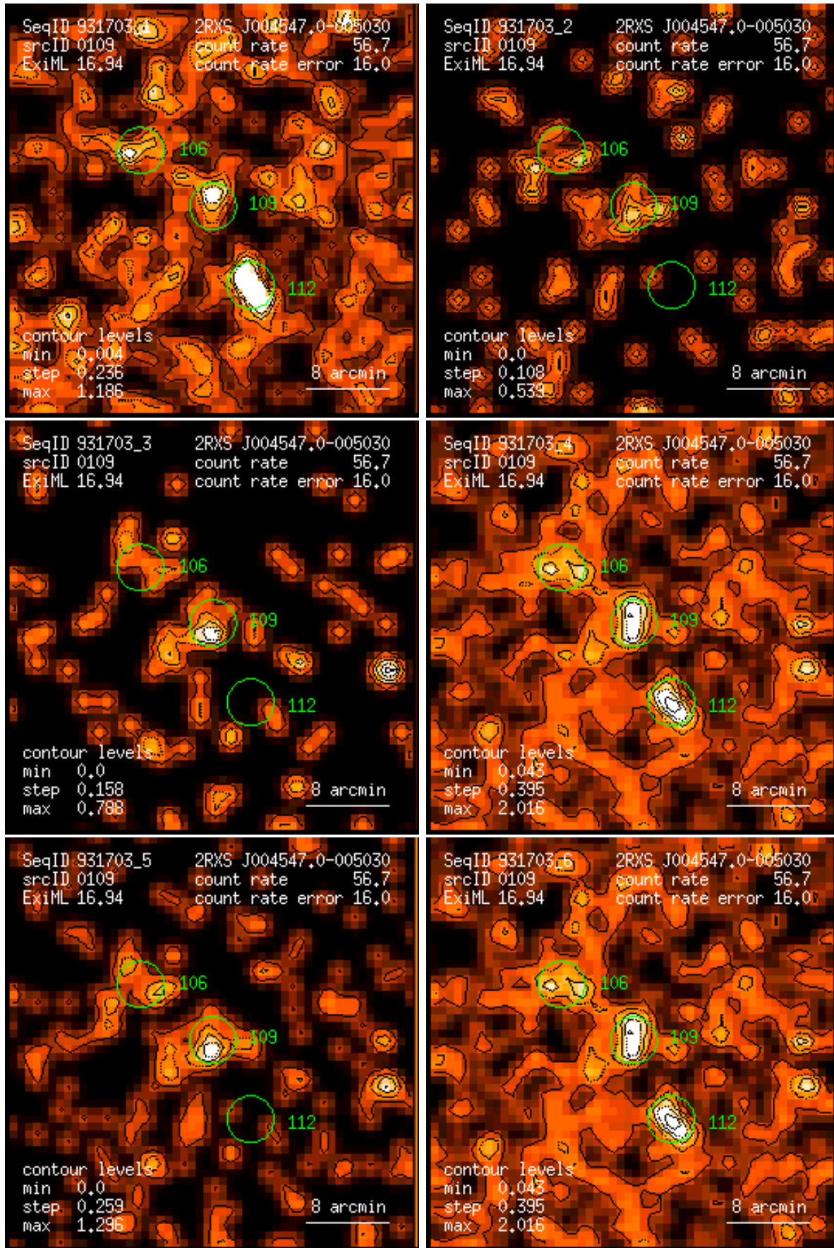
Figure 109: RASS 931703: detection 0109: band rate images, Gaussian filter: (1) PSPC channels 11 – 41, (2) 52 – 90, (3) 91 – 201, (4) 11 – 235, (5) 52 – 201, (6) 11 – 201. Broad band rates in counts/ks. Band rate contour levels in counts/ks/arcmin 2 .
