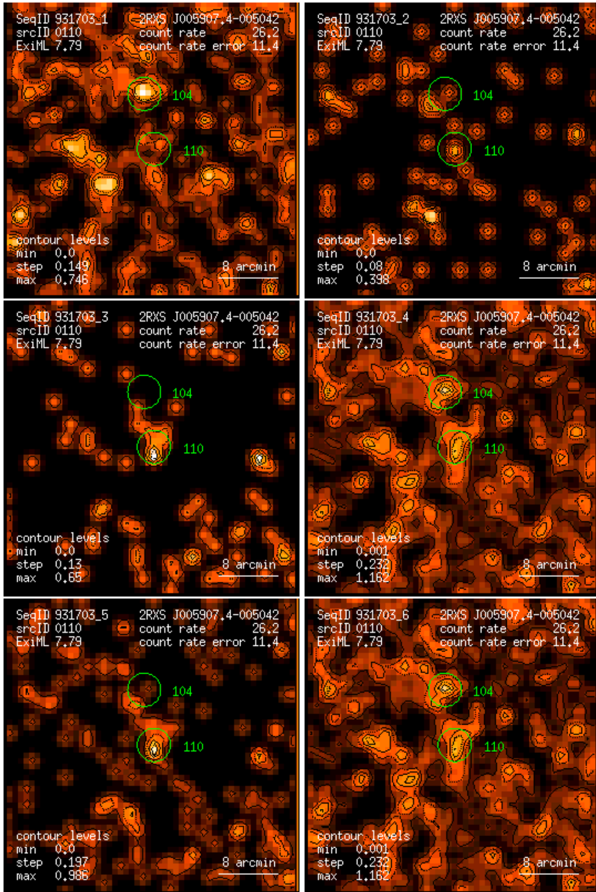
Figure 110: RASS 931703: detection 0110: band rate images, Gaussian filter: (1) PSPC channels 11 – 41, (2) 52 – 90, (3) 91 – 201, (4) 11 – 235, (5) 52 – 201, (6) 11 – 201. Broad band rates in counts/ks. Band rate contour levels in counts/ks/arcmin 2 .
