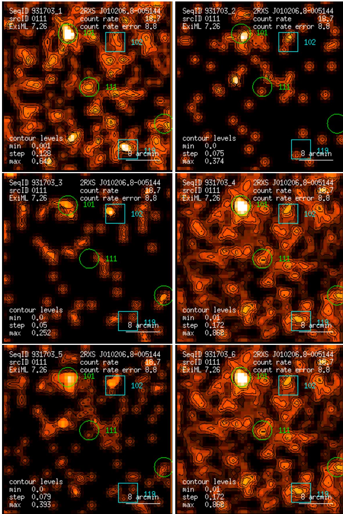
Figure 111: RASS 931703: detection 0111: band rate images, Gaussian filter: (1) PSPC channels 11 – 41, (2) 52 – 90, (3) 91 – 201, (4) 11 – 235, (5) 52 – 201, (6) 11 – 201. Broad band rates in counts/ks. Band rate contour levels in counts/ks/arcmin 2 .
