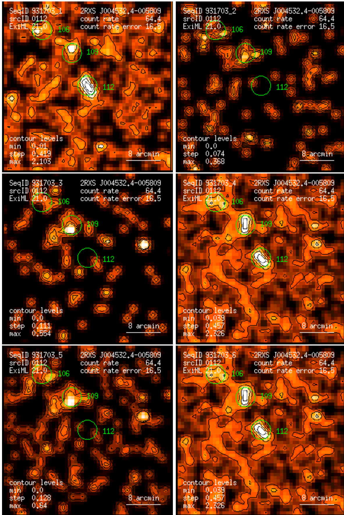
Figure 112: RASS 931703: detection 0112: band rate images, Gaussian filter: (1) PSPC channels 11 – 41, (2) 52 – 90, (3) 91 – 201, (4) 11 – 235, (5) 52 – 201, (6) 11 – 201. Broad band rates in counts/ks. Band rate contour levels in counts/ks/arcmin 2 .
