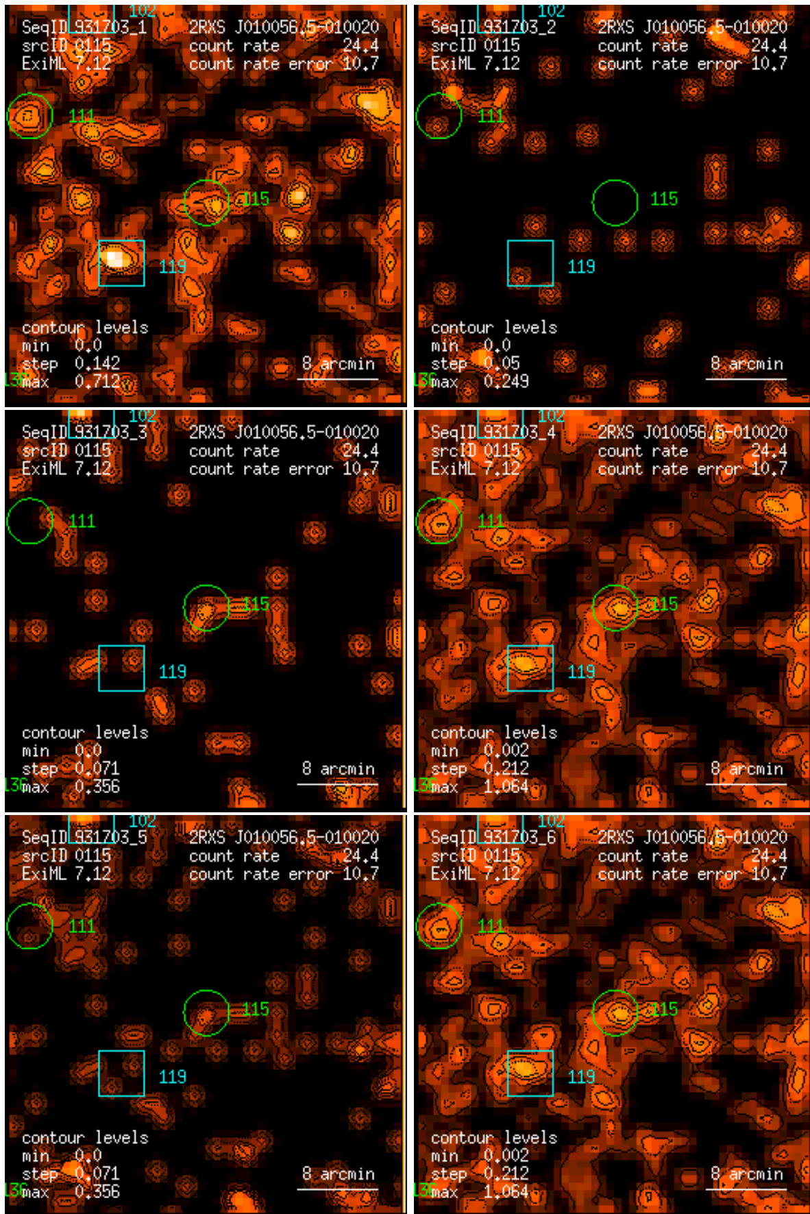
Figure 115: RASS 931703: detection 0115: band rate images, Gaussian filter: (1) PSPC channels 11 – 41, (2) 52 – 90, (3) 91 – 201, (4) 11 – 235, (5) 52 – 201, (6) 11 – 201. Broad band rates in counts/ks. Band rate contour levels in counts/ks/arcmin 2 .
