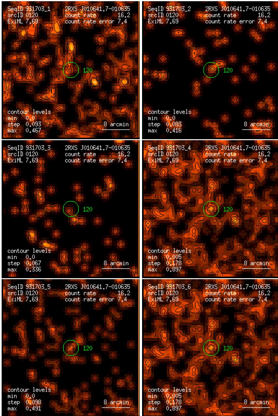
Figure 120: RASS 931703: detection 0120: band rate images, Gaussian filter: (1) PSPC channels 11 – 41, (2) 52 – 90, (3) 91 – 201, (4) 11 – 235, (5) 52 – 201, (6) 11 – 201. Broad band rates in counts/ks. Band rate contour levels in counts/ks/arcmin 2 .
