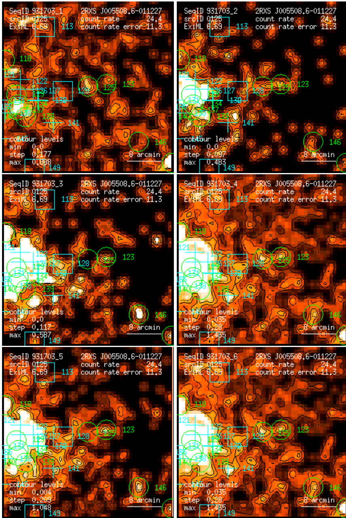
Figure 125: RASS 931703: detection 0125: band rate images, Gaussian filter: (1) PSPC channels 11 – 41, (2) 52 – 90, (3) 91 – 201, (4) 11 – 235, (5) 52 – 201, (6) 11 – 201. Broad band rates in counts/ks. Band rate contour levels in counts/ks/arcmin 2 .
